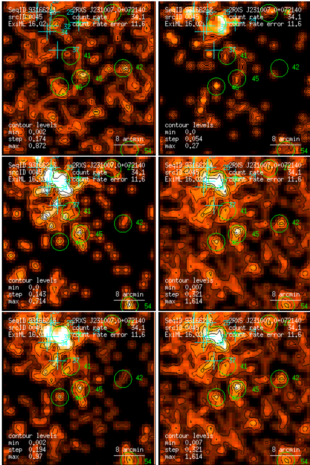
Figure 45: RASS 931662: detection 0045: band rate images, Gaussian filter: (1) PSPC channels 11 – 41, (2) 52 – 90, (3) 91 – 201, (4) 11 – 235, (5) 52 – 201, (6) 11 – 201. Broad band rates in counts/ks. Band rate contour levels in counts/ks/arcmin 2 .
