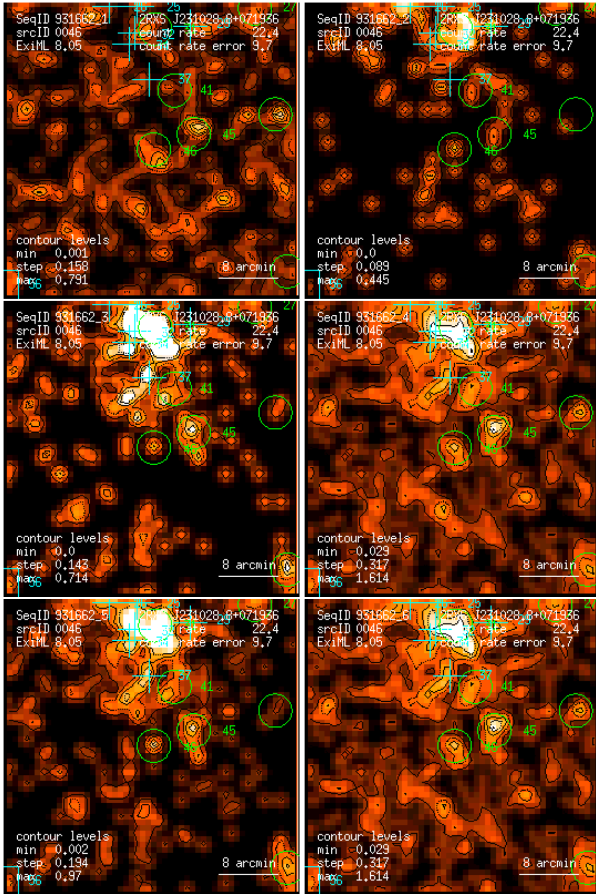
Figure 46: RASS 931662: detection 0046: band rate images, Gaussian filter: (1) PSPC channels 11 – 41, (2) 52 – 90, (3) 91 – 201, (4) 11 – 235, (5) 52 – 201, (6) 11 – 201. Broad band rates in counts/ks. Band rate contour levels in counts/ks/arcmin 2 .
