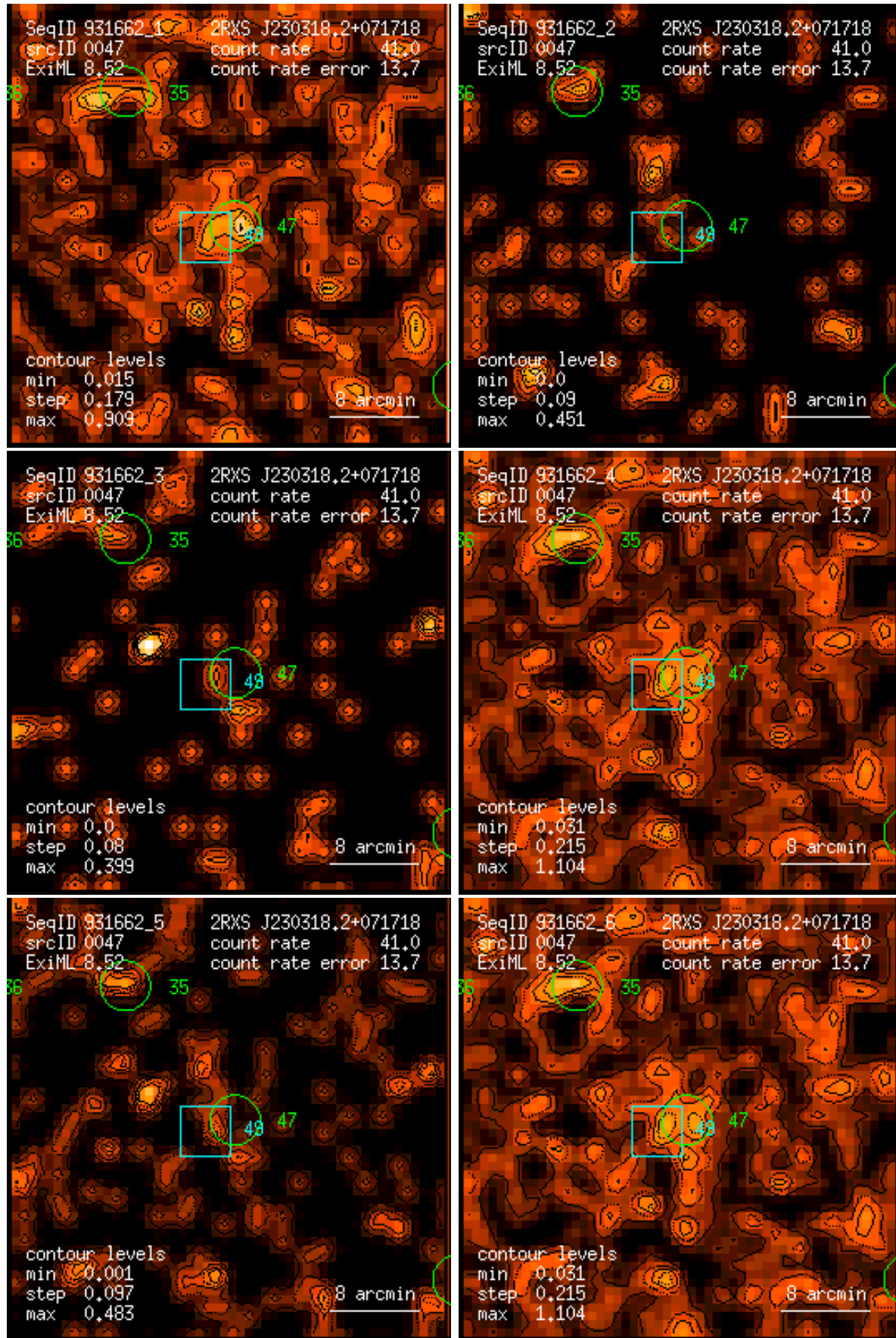
Figure 47: RASS 931662: detection 0047: band rate images, Gaussian filter: (1) PSPC channels 11 – 41, (2) 52 – 90, (3) 91 – 201, (4) 11 – 235, (5) 52 – 201, (6) 11 – 201. Broad band rates in counts/ks. Band rate contour levels in counts/ks/arcmin 2 .
