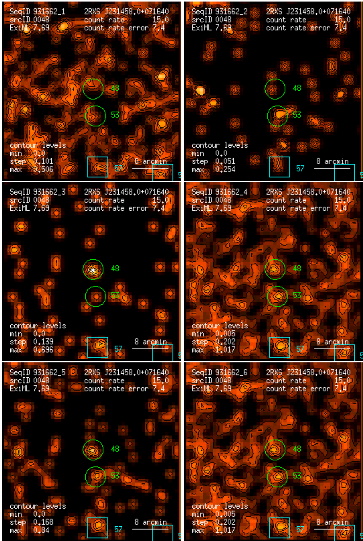
Figure 48: RASS 931662: detection 0048: band rate images, Gaussian filter: (1) PSPC channels 11 – 41, (2) 52 – 90, (3) 91 – 201, (4) 11 – 235, (5) 52 – 201, (6) 11 – 201. Broad band rates in counts/ks. Band rate contour levels in counts/ks/arcmin 2 .
