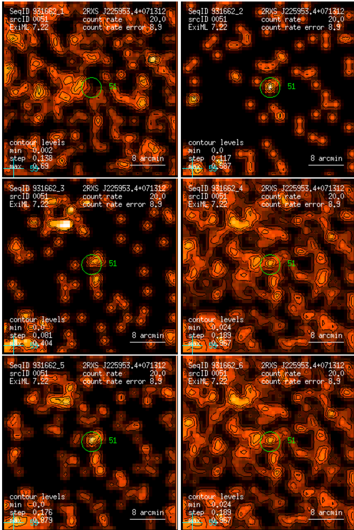
Figure 51: RASS 931662: detection 0051: band rate images, Gaussian filter: (1) PSPC channels 11 – 41, (2) 52 – 90, (3) 91 – 201, (4) 11 – 235, (5) 52 – 201, (6) 11 – 201. Broad band rates in counts/ks. Band rate contour levels in counts/ks/arcmin 2 .
