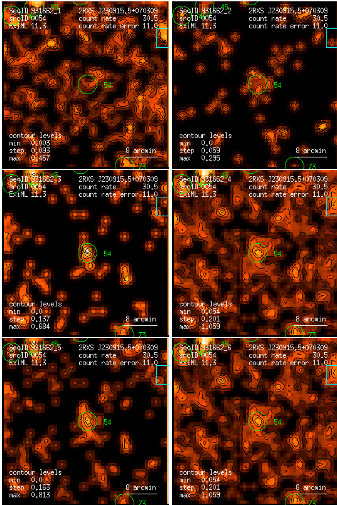
Figure 54: RASS 931662: detection 0054: band rate images, Gaussian filter: (1) PSPC channels 11 – 41, (2) 52 – 90, (3) 91 – 201, (4) 11 – 235, (5) 52 – 201, (6) 11 – 201. Broad band rates in counts/ks. Band rate contour levels in counts/ks/arcmin 2 .
