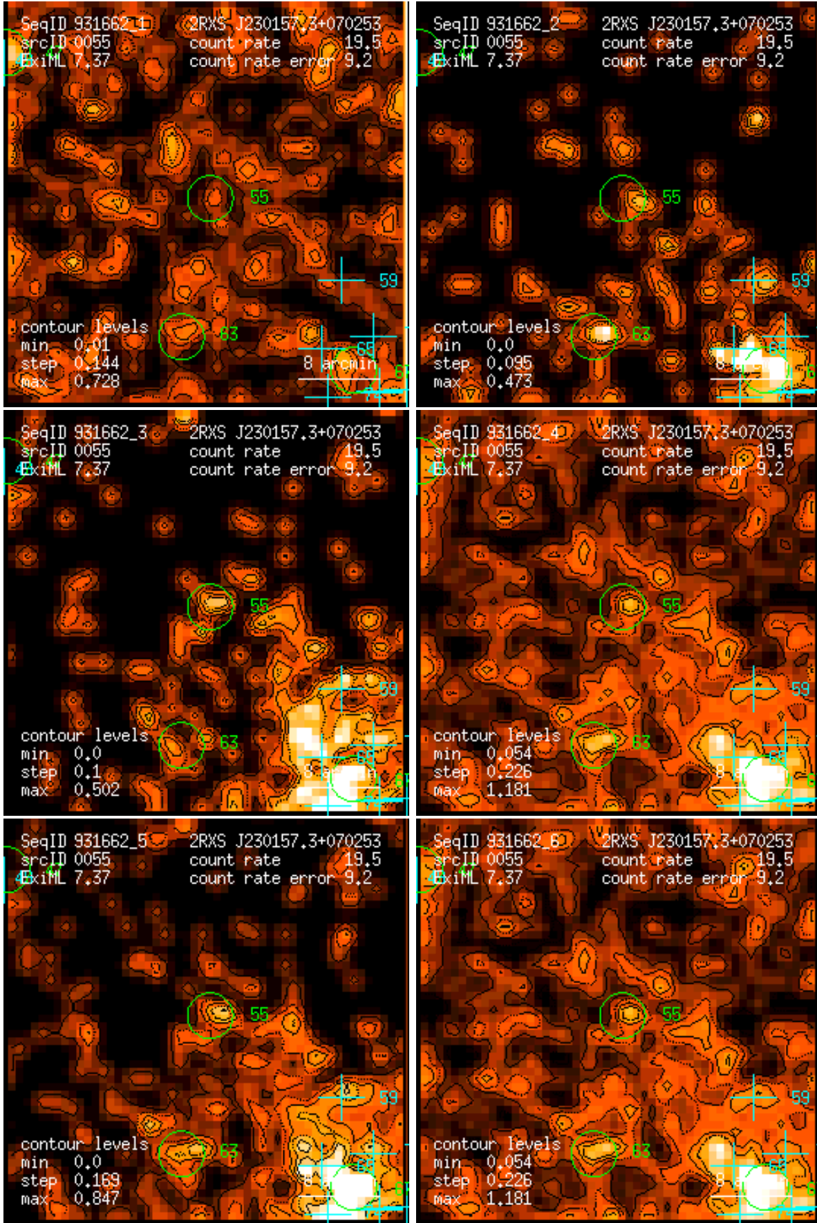
Figure 55: RASS 931662: detection 0055: band rate images, Gaussian filter: (1) PSPC channels 11 – 41, (2) 52 – 90, (3) 91 – 201, (4) 11 – 235, (5) 52 – 201, (6) 11 – 201. Broad band rates in counts/ks. Band rate contour levels in counts/ks/arcmin 2 .
