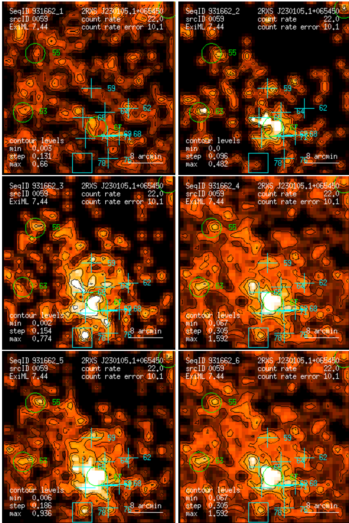
Figure 59: RASS 931662: detection 0059: band rate images, Gaussian filter: (1) PSPC channels 11 – 41, (2) 52 – 90, (3) 91 – 201, (4) 11 – 235, (5) 52 – 201, (6) 11 – 201. Broad band rates in counts/ks. Band rate contour levels in counts/ks/arcmin 2 .
