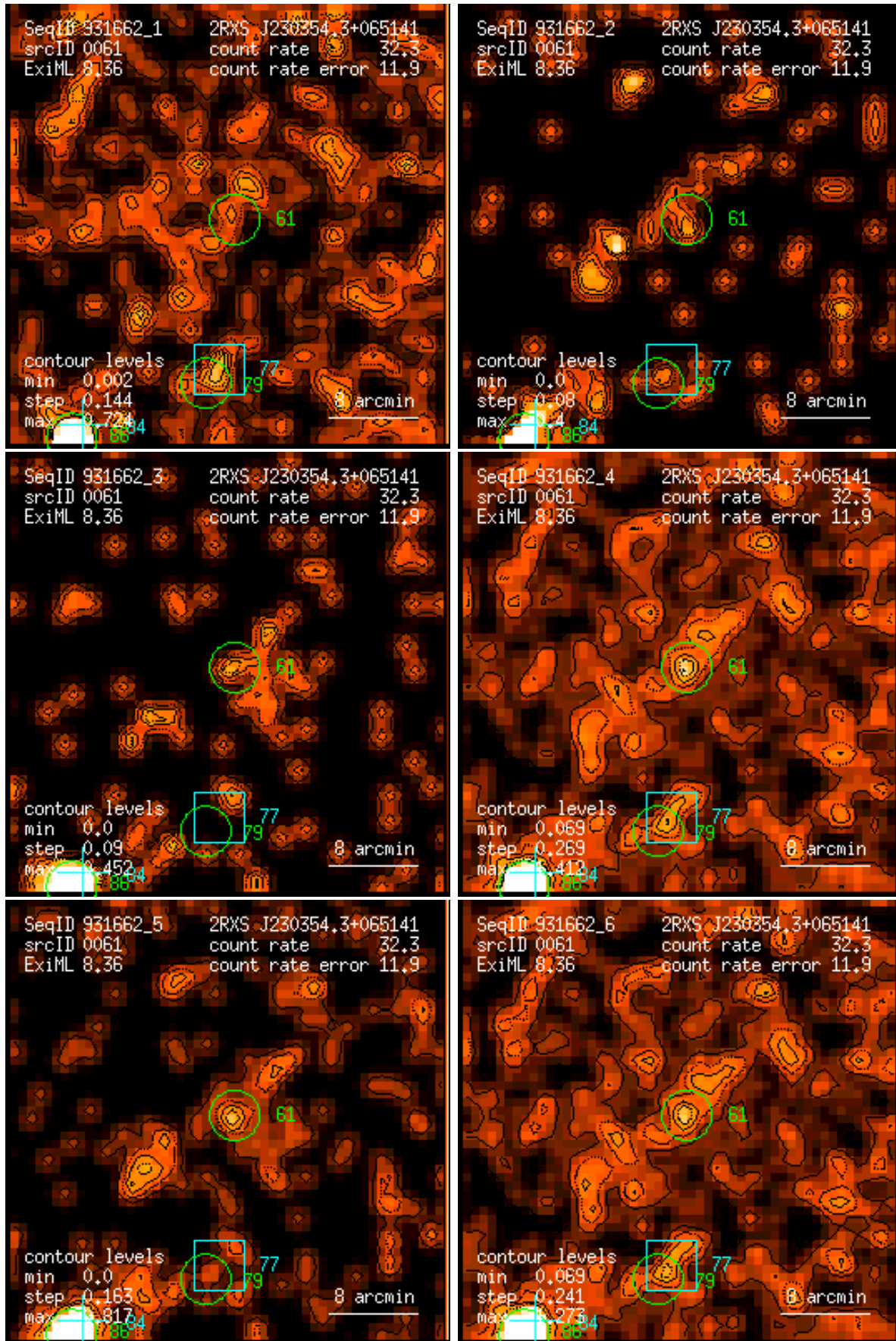
Figure 61: RASS 931662: detection 0061: band rate images, Gaussian filter: (1) PSPC channels 11 – 41, (2) 52 – 90, (3) 91 – 201, (4) 11 – 235, (5) 52 – 201, (6) 11 – 201. Broad band rates in counts/ks. Band rate contour levels in counts/ks/arcmin 2 .
