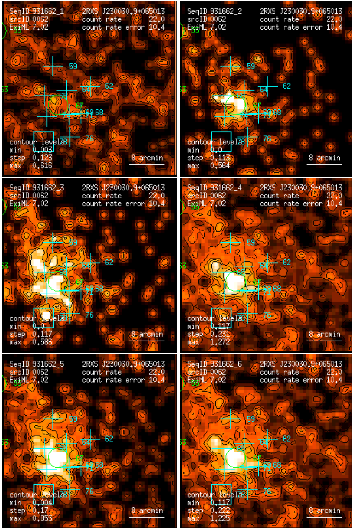
Figure 62: RASS 931662: detection 0062: band rate images, Gaussian filter: (1) PSPC channels 11 – 41, (2) 52 – 90, (3) 91 – 201, (4) 11 – 235, (5) 52 – 201, (6) 11 – 201. Broad band rates in counts/ks. Band rate contour levels in counts/ks/arcmin 2 .
