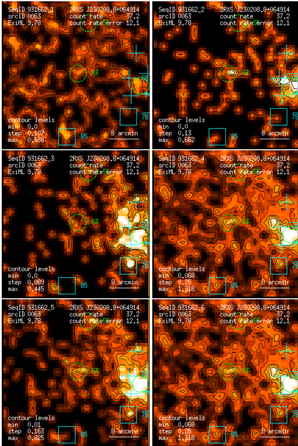
Figure 63: RASS 931662: detection 0063: band rate images, Gaussian filter: (1) PSPC channels 11 – 41, (2) 52 – 90, (3) 91 – 201, (4) 11 – 235, (5) 52 – 201, (6) 11 – 201. Broad band rates in counts/ks. Band rate contour levels in counts/ks/arcmin 2 .
