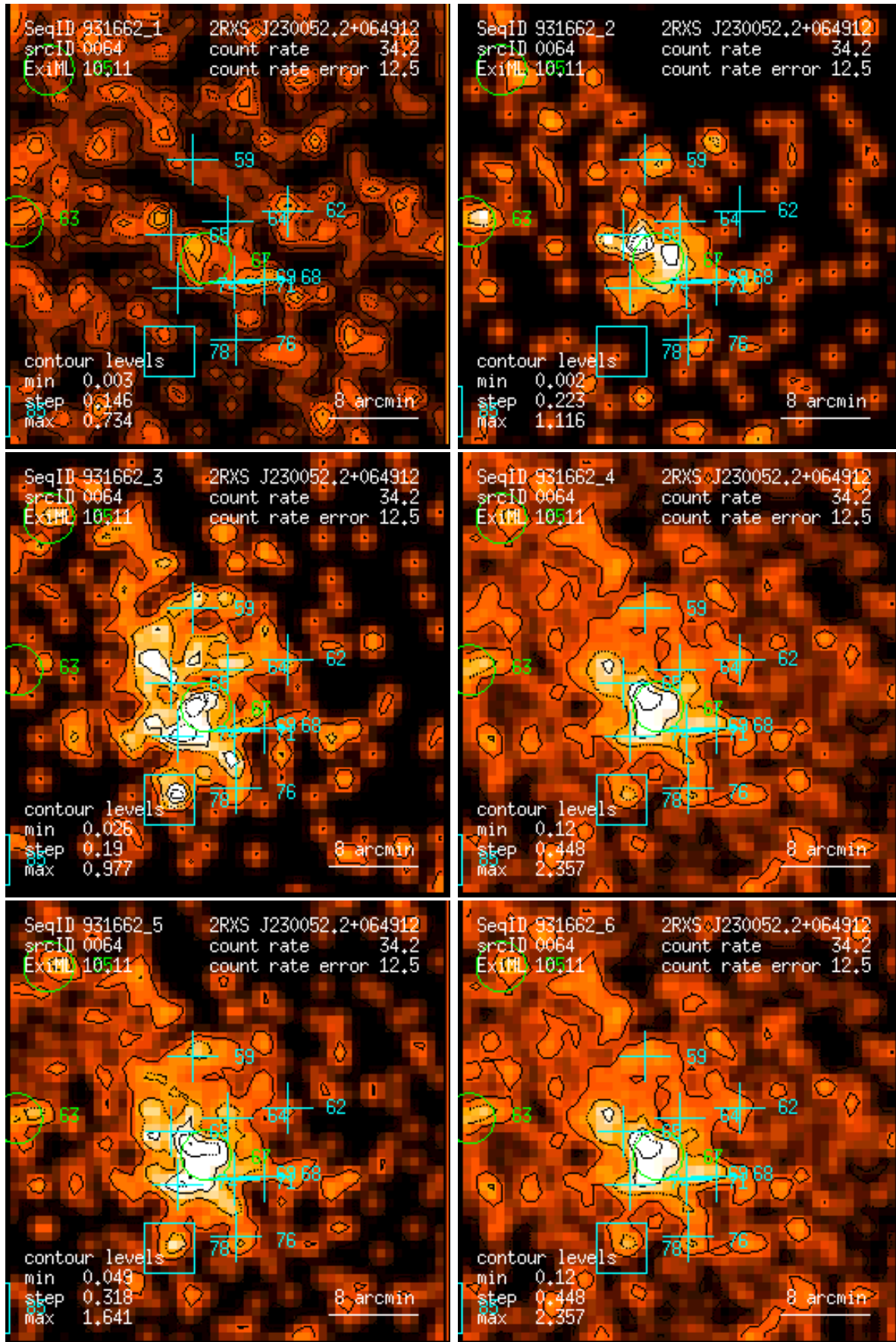
Figure 64: RASS 931662: detection 0064: band rate images, Gaussian filter: (1) PSPC channels 11 – 41, (2) 52 – 90, (3) 91 – 201, (4) 11 – 235, (5) 52 – 201, (6) 11 – 201. Broad band rates in counts/ks. Band rate contour levels in counts/ks/arcmin 2 .
