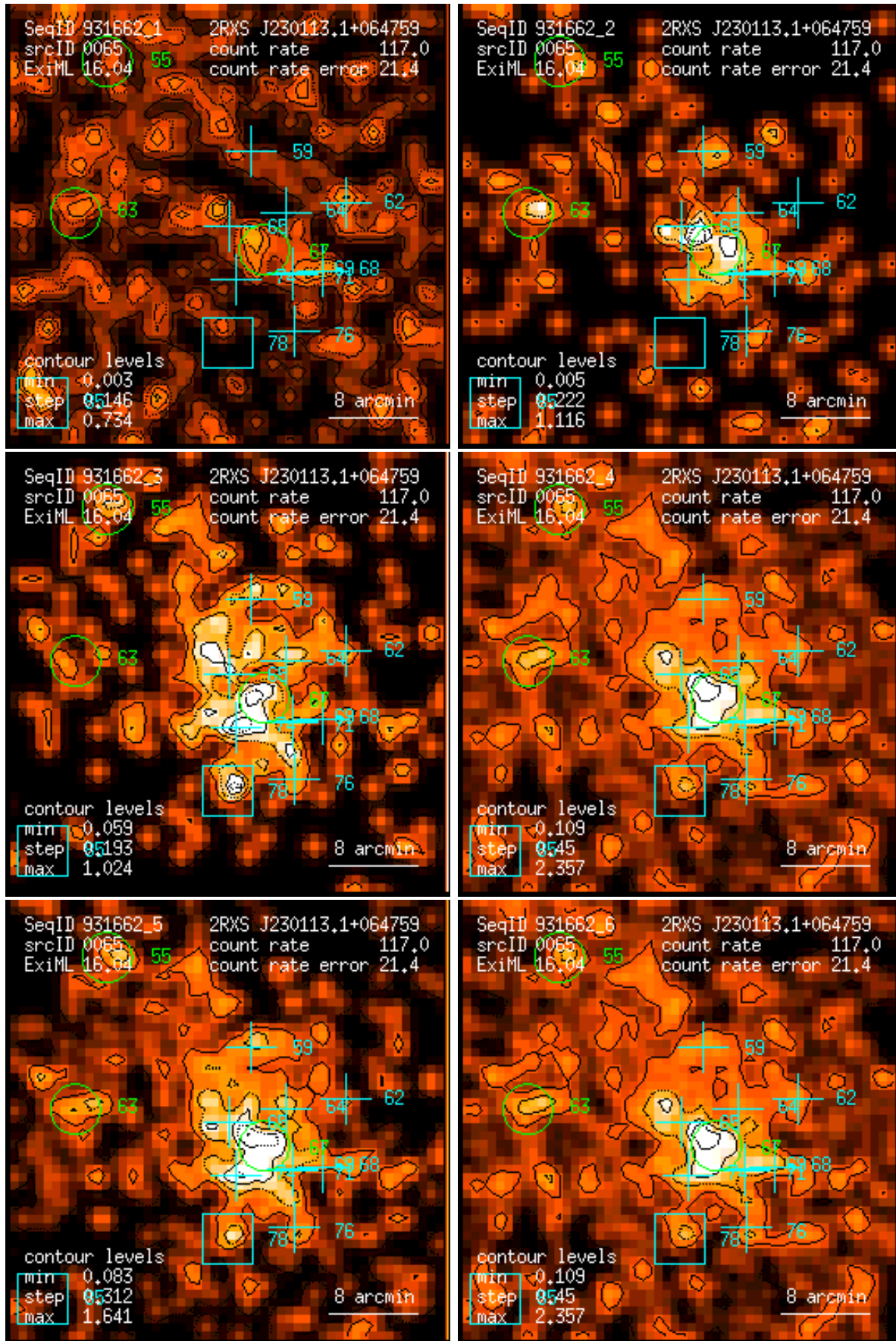
Figure 65: RASS 931662: detection 0065: band rate images, Gaussian filter: (1) PSPC channels 11 – 41, (2) 52 – 90, (3) 91 – 201, (4) 11 – 235, (5) 52 – 201, (6) 11 – 201. Broad band rates in counts/ks. Band rate contour levels in counts/ks/arcmin 2 .
