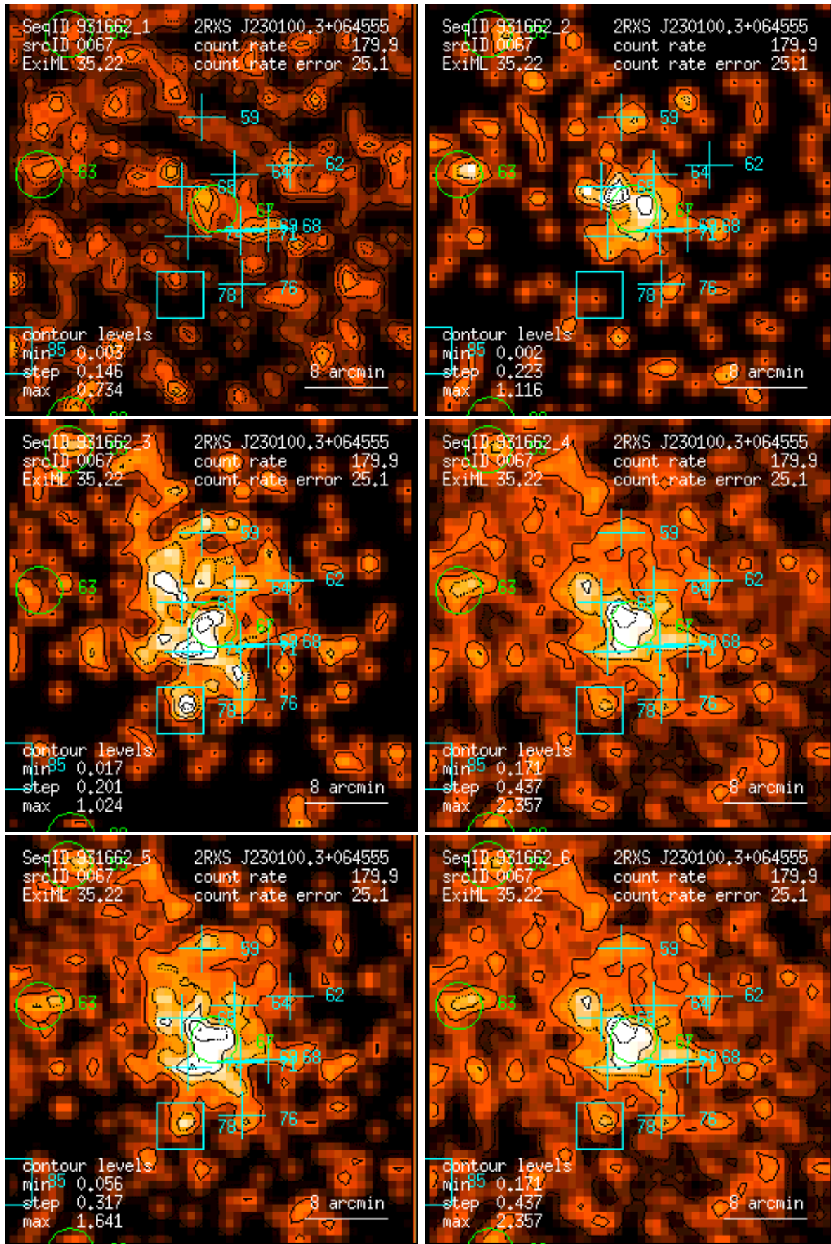
Figure 67: RASS 931662: detection 0067: band rate images, Gaussian filter: (1) PSPC channels 11 – 41, (2) 52 – 90, (3) 91 – 201, (4) 11 – 235, (5) 52 – 201, (6) 11 – 201. Broad band rates in counts/ks. Band rate contour levels in counts/ks/arcmin 2 .
