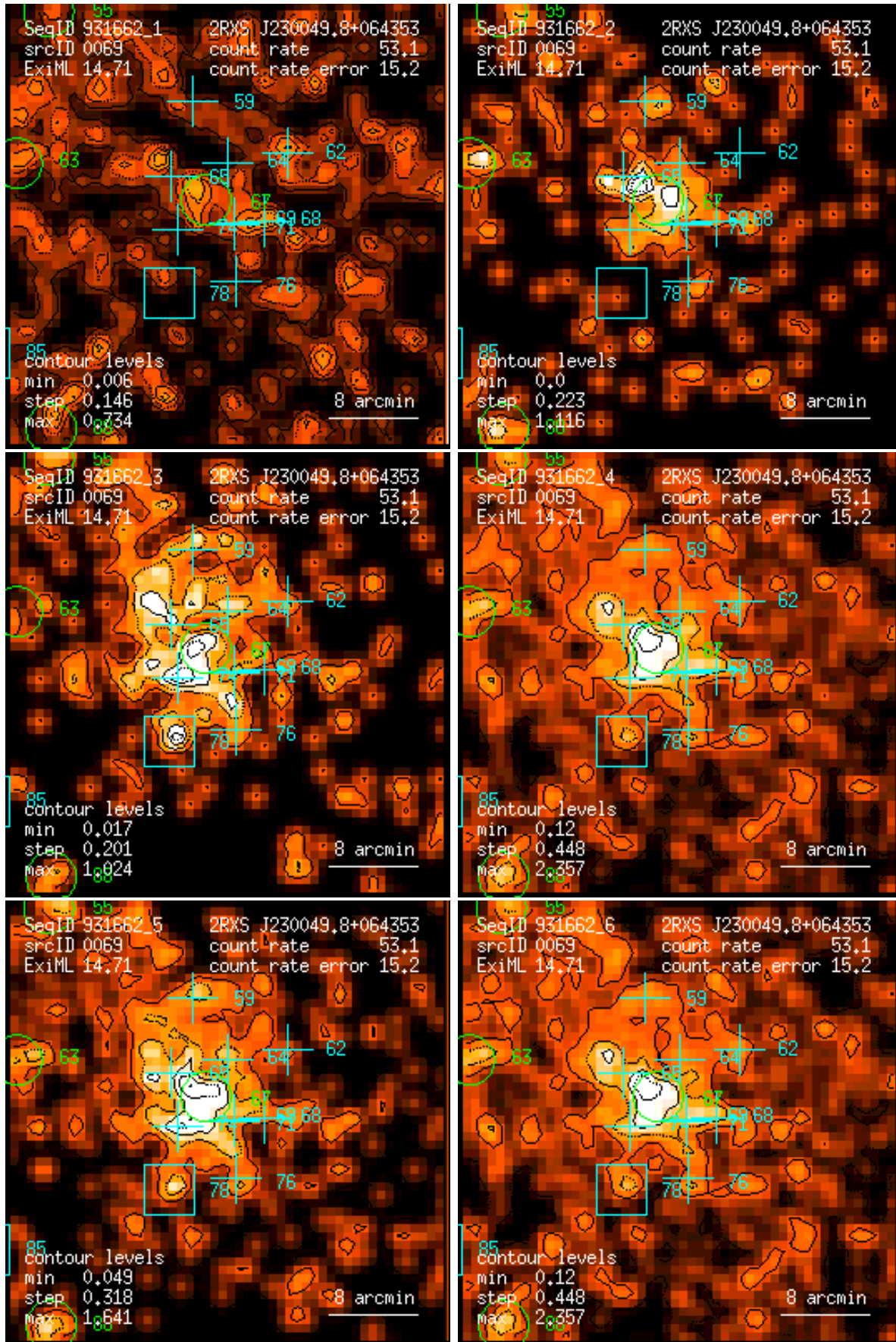
Figure 69: RASS 931662: detection 0069: band rate images, Gaussian filter: (1) PSPC channels 11 – 41, (2) 52 – 90, (3) 91 – 201, (4) 11 – 235, (5) 52 – 201, (6) 11 – 201. Broad band rates in counts/ks. Band rate contour levels in counts/ks/arcmin 2 .
