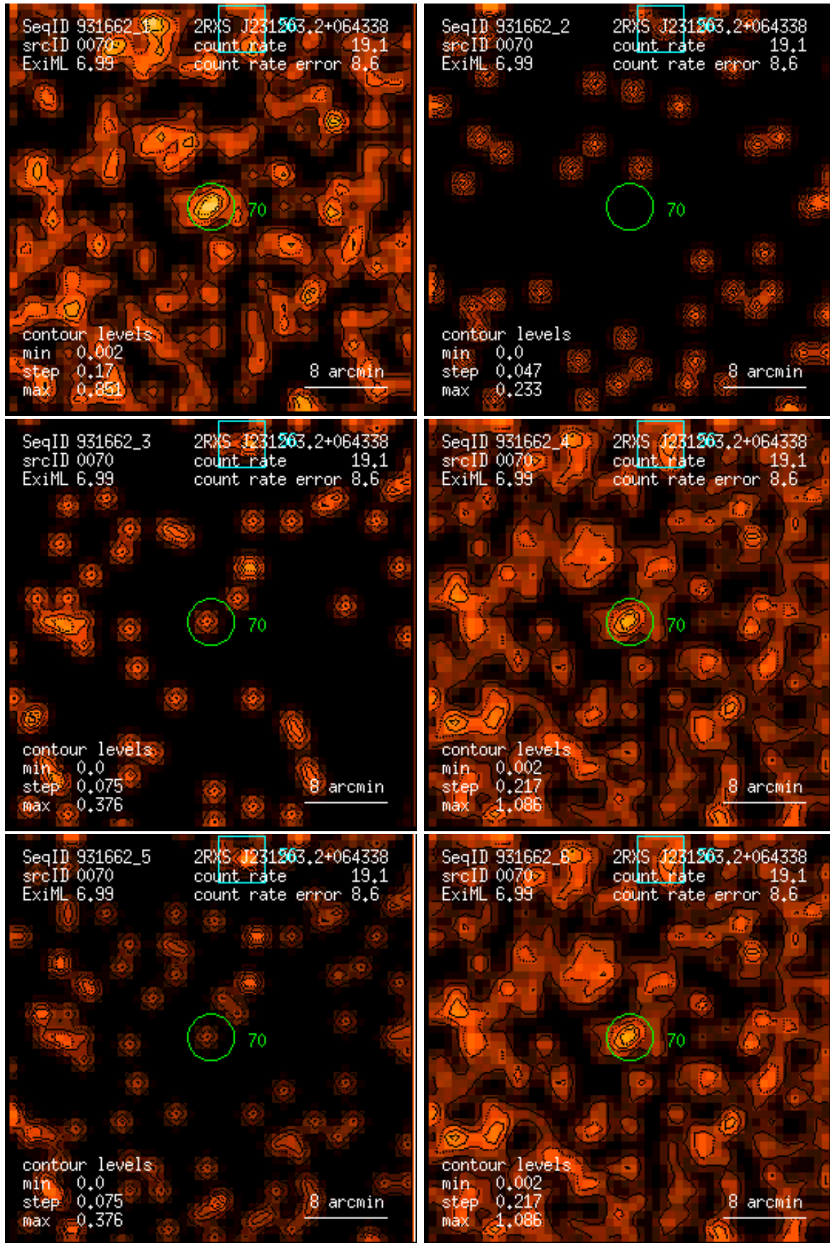
Figure 70: RASS 931662: detection 0070: band rate images, Gaussian filter: (1) PSPC channels 11 – 41, (2) 52 – 90, (3) 91 – 201, (4) 11 – 235, (5) 52 – 201, (6) 11 – 201. Broad band rates in counts/ks. Band rate contour levels in counts/ks/arcmin 2 .
