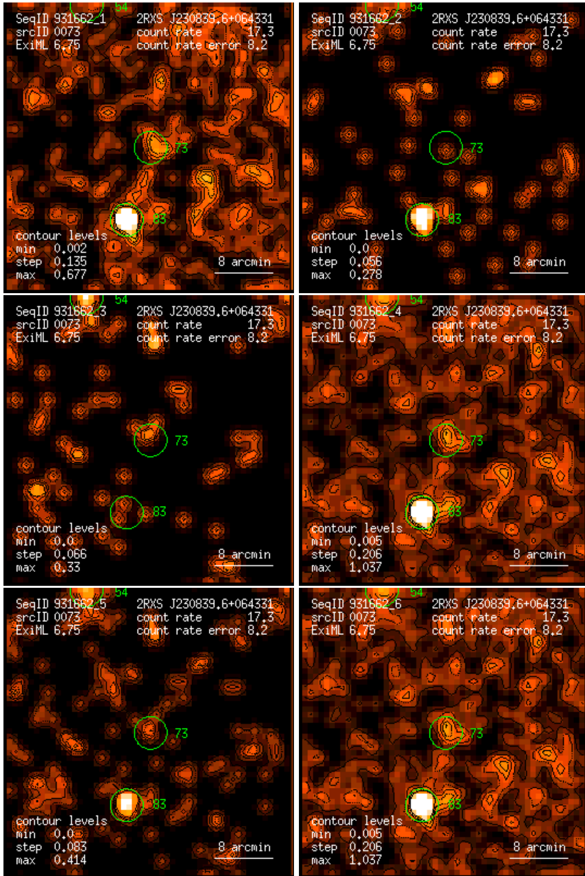
Figure 73: RASS 931662: detection 0073: band rate images, Gaussian filter: (1) PSPC channels 11 – 41, (2) 52 – 90, (3) 91 – 201, (4) 11 – 235, (5) 52 – 201, (6) 11 – 201. Broad band rates in counts/ks. Band rate contour levels in counts/ks/arcmin 2 .
