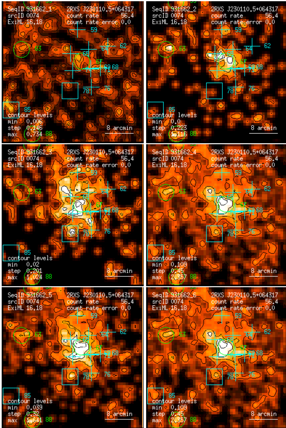
Figure 74: RASS 931662: detection 0074: band rate images, Gaussian filter: (1) PSPC channels 11 – 41, (2) 52 – 90, (3) 91 – 201, (4) 11 – 235, (5) 52 – 201, (6) 11 – 201. Broad band rates in counts/ks. Band rate contour levels in counts/ks/arcmin 2 .
