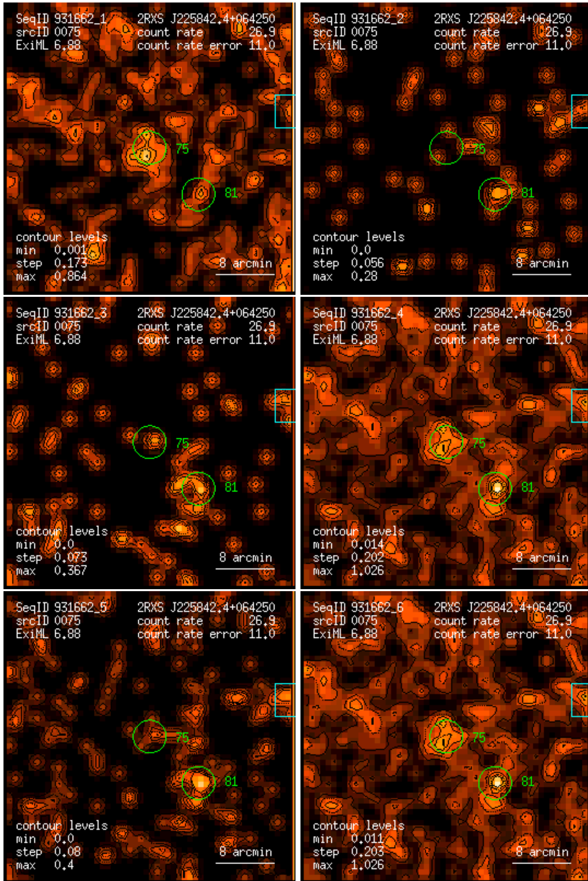
Figure 75: RASS 931662: detection 0075: band rate images, Gaussian filter: (1) PSPC channels 11 – 41, (2) 52 – 90, (3) 91 – 201, (4) 11 – 235, (5) 52 – 201, (6) 11 – 201. Broad band rates in counts/ks. Band rate contour levels in counts/ks/arcmin 2 .
