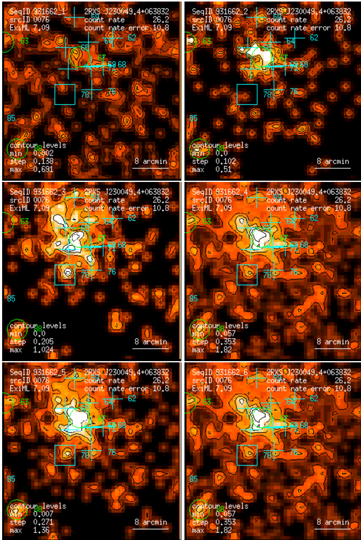
Figure 76: RASS 931662: detection 0076: band rate images, Gaussian filter: (1) PSPC channels 11 – 41, (2) 52 – 90, (3) 91 – 201, (4) 11 – 235, (5) 52 – 201, (6) 11 – 201. Broad band rates in counts/ks. Band rate contour levels in counts/ks/arcmin 2 .
