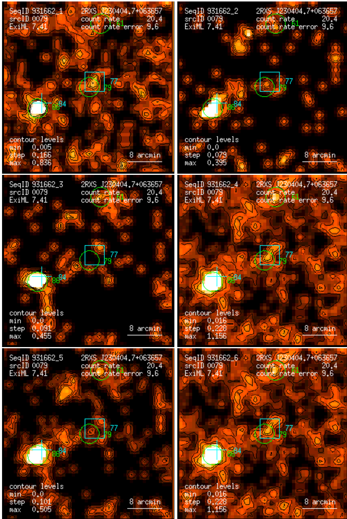
Figure 79: RASS 931662: detection 0079: band rate images, Gaussian filter: (1) PSPC channels 11 – 41, (2) 52 – 90, (3) 91 – 201, (4) 11 – 235, (5) 52 – 201, (6) 11 – 201. Broad band rates in counts/ks. Band rate contour levels in counts/ks/arcmin 2 .
