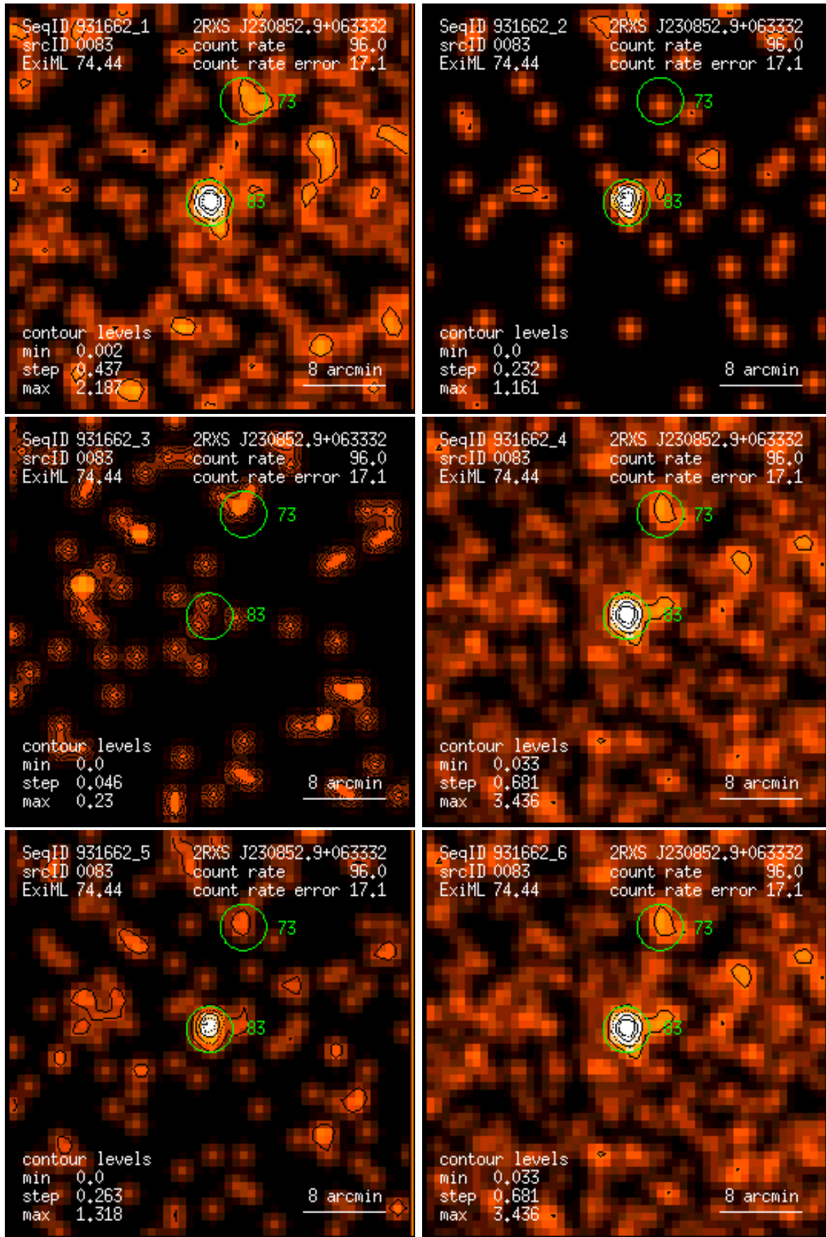
Figure 83: RASS 931662: detection 0083: band rate images, Gaussian filter: (1) PSPC channels 11 – 41, (2) 52 – 90, (3) 91 – 201, (4) 11 – 235, (5) 52 – 201, (6) 11 – 201. Broad band rates in counts/ks. Band rate contour levels in counts/ks/arcmin 2 .
