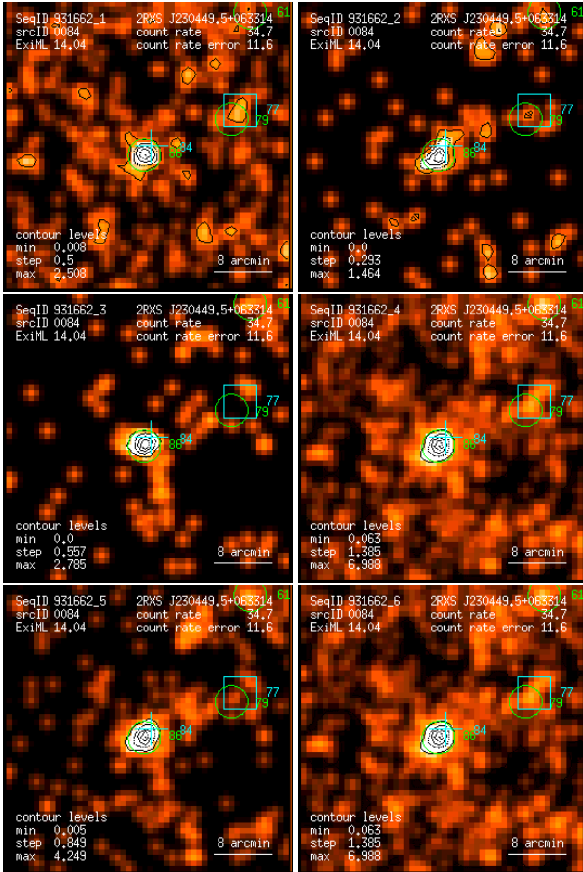
Figure 84: RASS 931662: detection 0084: band rate images, Gaussian filter: (1) PSPC channels 11 – 41, (2) 52 – 90, (3) 91 – 201, (4) 11 – 235, (5) 52 – 201, (6) 11 – 201. Broad band rates in counts/ks. Band rate contour levels in counts/ks/arcmin 2 .
