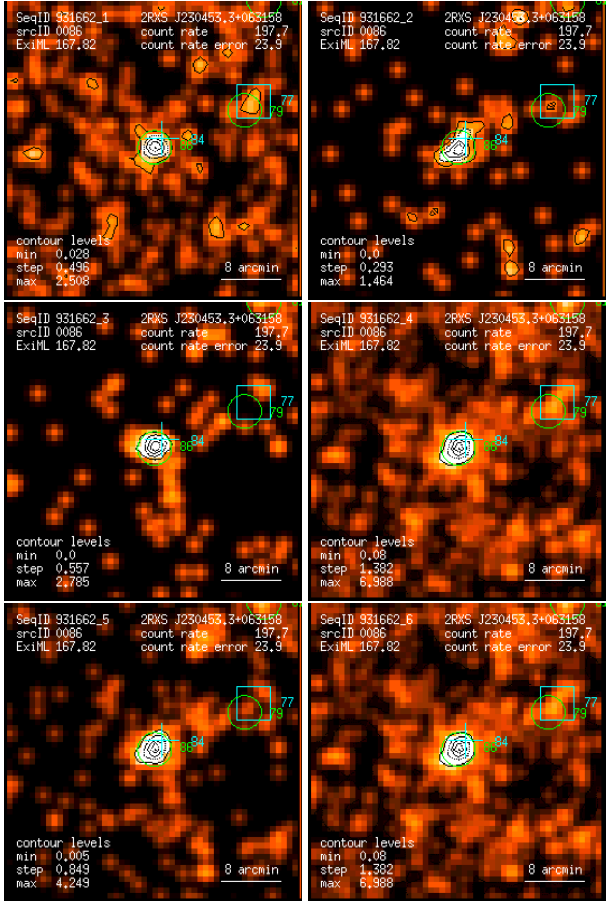
Figure 86: RASS 931662: detection 0086: band rate images, Gaussian filter: (1) PSPC channels 11 – 41, (2) 52 – 90, (3) 91 – 201, (4) 11 – 235, (5) 52 – 201, (6) 11 – 201. Broad band rates in counts/ks. Band rate contour levels in counts/ks/arcmin 2 .
