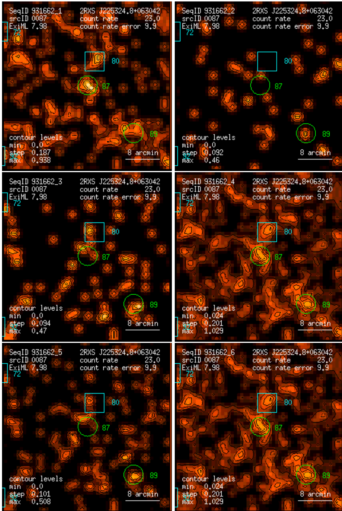
Figure 87: RASS 931662: detection 0087: band rate images, Gaussian filter: (1) PSPC channels 11 – 41, (2) 52 – 90, (3) 91 – 201, (4) 11 – 235, (5) 52 – 201, (6) 11 – 201. Broad band rates in counts/ks. Band rate contour levels in counts/ks/arcmin 2 .
