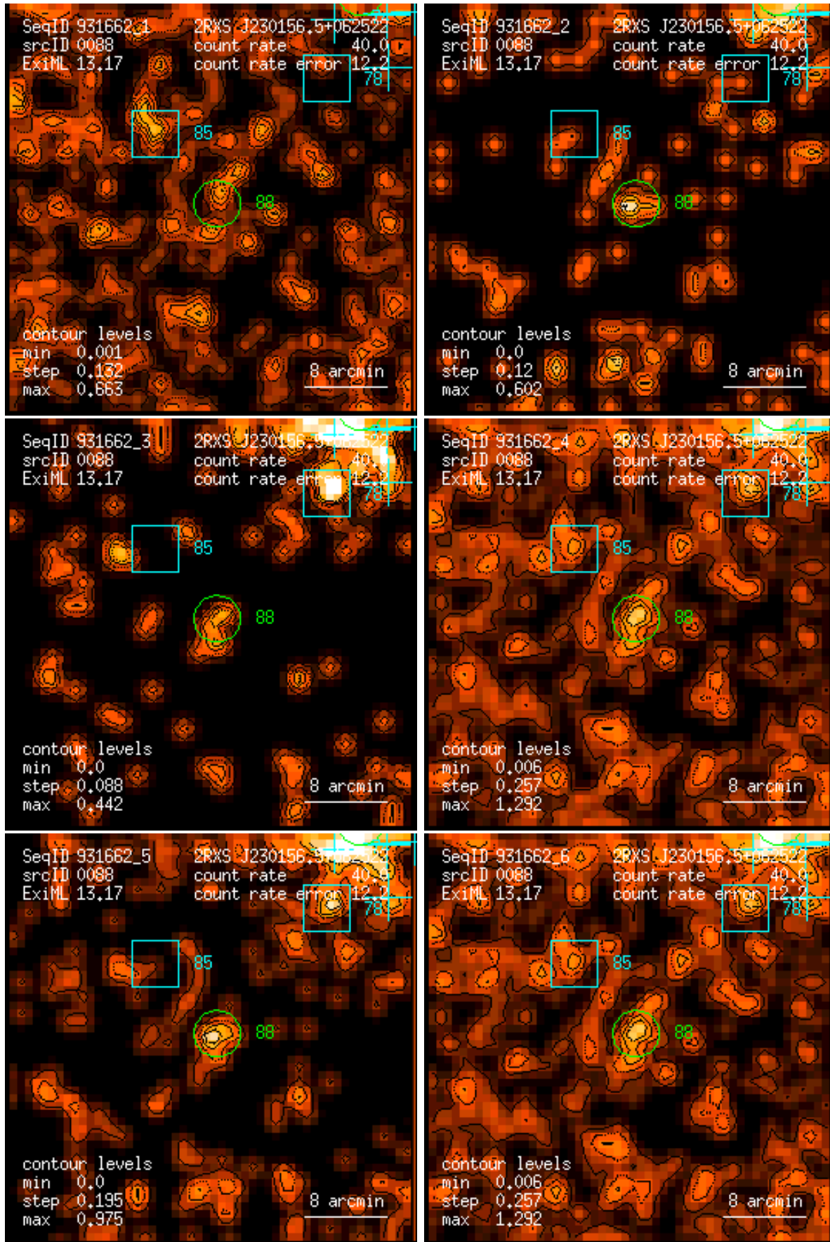
Figure 88: RASS 931662: detection 0088: band rate images, Gaussian filter: (1) PSPC channels 11 – 41, (2) 52 – 90, (3) 91 – 201, (4) 11 – 235, (5) 52 – 201, (6) 11 – 201. Broad band rates in counts/ks. Band rate contour levels in counts/ks/arcmin 2 .
