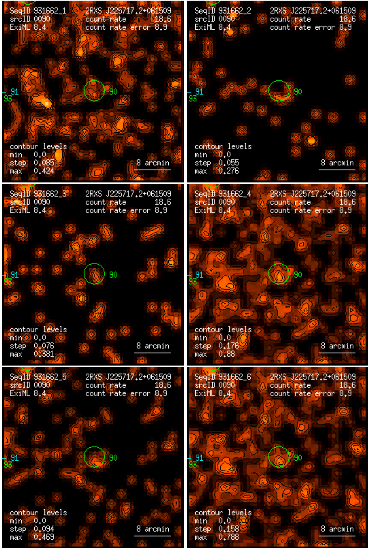
Figure 90: RASS 931662: detection 0090: band rate images, Gaussian filter: (1) PSPC channels 11 – 41, (2) 52 – 90, (3) 91 – 201, (4) 11 – 235, (5) 52 – 201, (6) 11 – 201. Broad band rates in counts/ks. Band rate contour levels in counts/ks/arcmin 2 .
