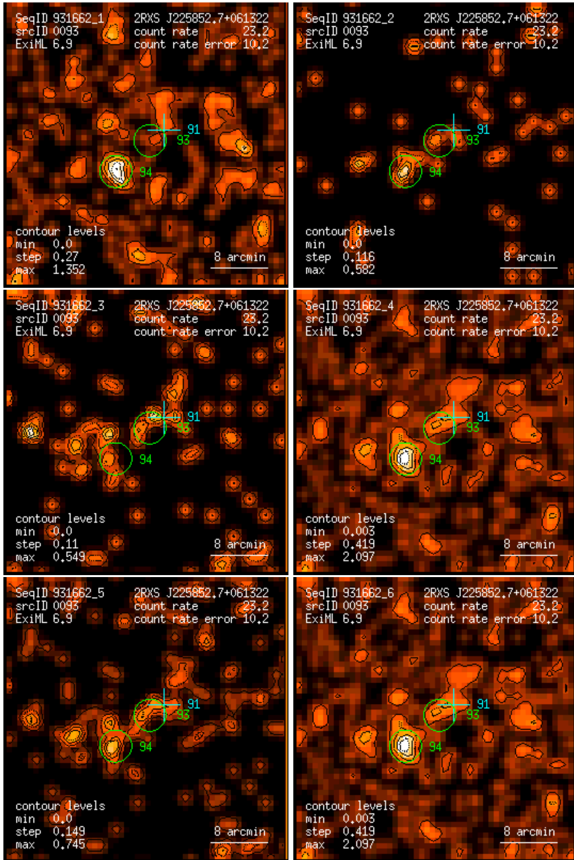
Figure 93: RASS 931662: detection 0093: band rate images, Gaussian filter: (1) PSPC channels 11 – 41, (2) 52 – 90, (3) 91 – 201, (4) 11 – 235, (5) 52 – 201, (6) 11 – 201. Broad band rates in counts/ks. Band rate contour levels in counts/ks/arcmin 2 .
