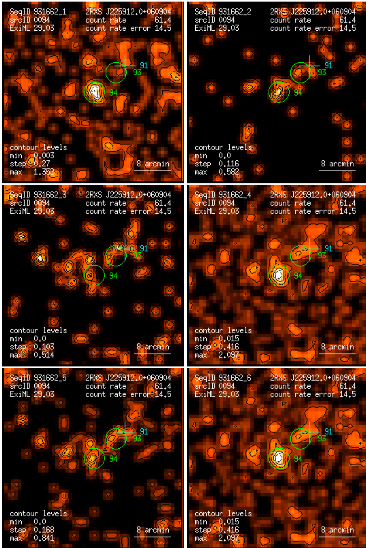
Figure 94: RASS 931662: detection 0094: band rate images, Gaussian filter: (1) PSPC channels 11 – 41, (2) 52 – 90, (3) 91 – 201, (4) 11 – 235, (5) 52 – 201, (6) 11 – 201. Broad band rates in counts/ks. Band rate contour levels in counts/ks/arcmin 2 .
