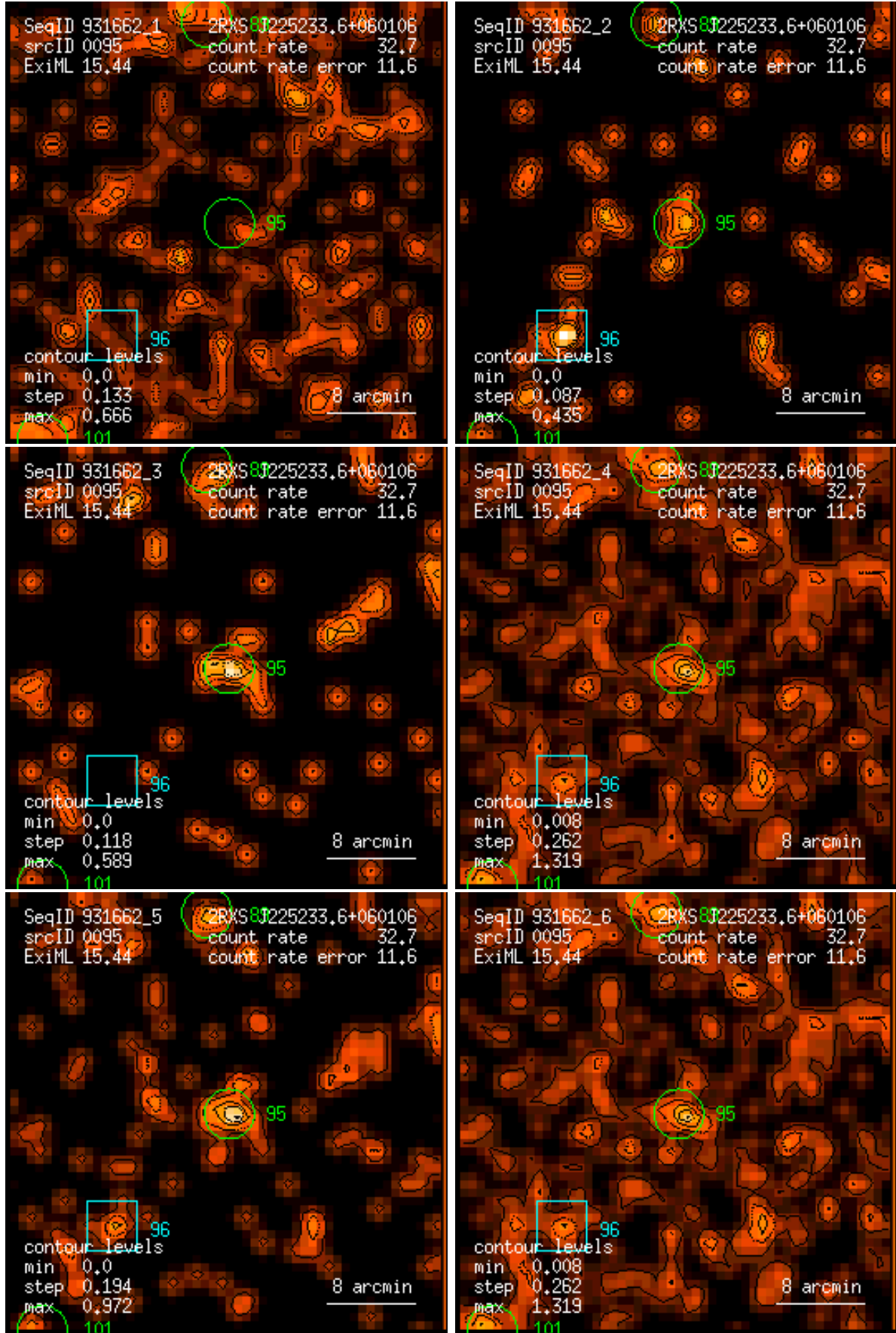
Figure 95: RASS 931662: detection 0095: band rate images, Gaussian filter: (1) PSPC channels 11 – 41, (2) 52 – 90, (3) 91 – 201, (4) 11 – 235, (5) 52 – 201, (6) 11 – 201. Broad band rates in counts/ks. Band rate contour levels in counts/ks/arcmin 2 .
