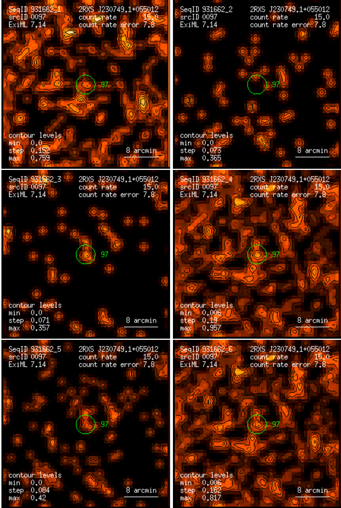
Figure 97: RASS 931662: detection 0097: band rate images, Gaussian filter: (1) PSPC channels 11 – 41, (2) 52 – 90, (3) 91 – 201, (4) 11 – 235, (5) 52 – 201, (6) 11 – 201. Broad band rates in counts/ks. Band rate contour levels in counts/ks/arcmin 2 .
