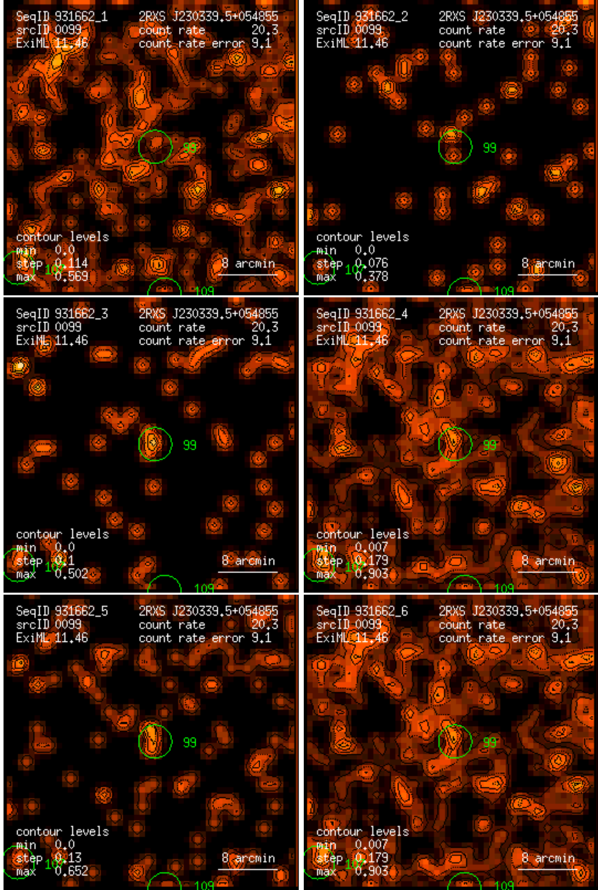
Figure 99: RASS 931662: detection 0099: band rate images, Gaussian filter: (1) PSPC channels 11 – 41, (2) 52 – 90, (3) 91 – 201, (4) 11 – 235, (5) 52 – 201, (6) 11 – 201. Broad band rates in counts/ks. Band rate contour levels in counts/ks/arcmin 2 .
