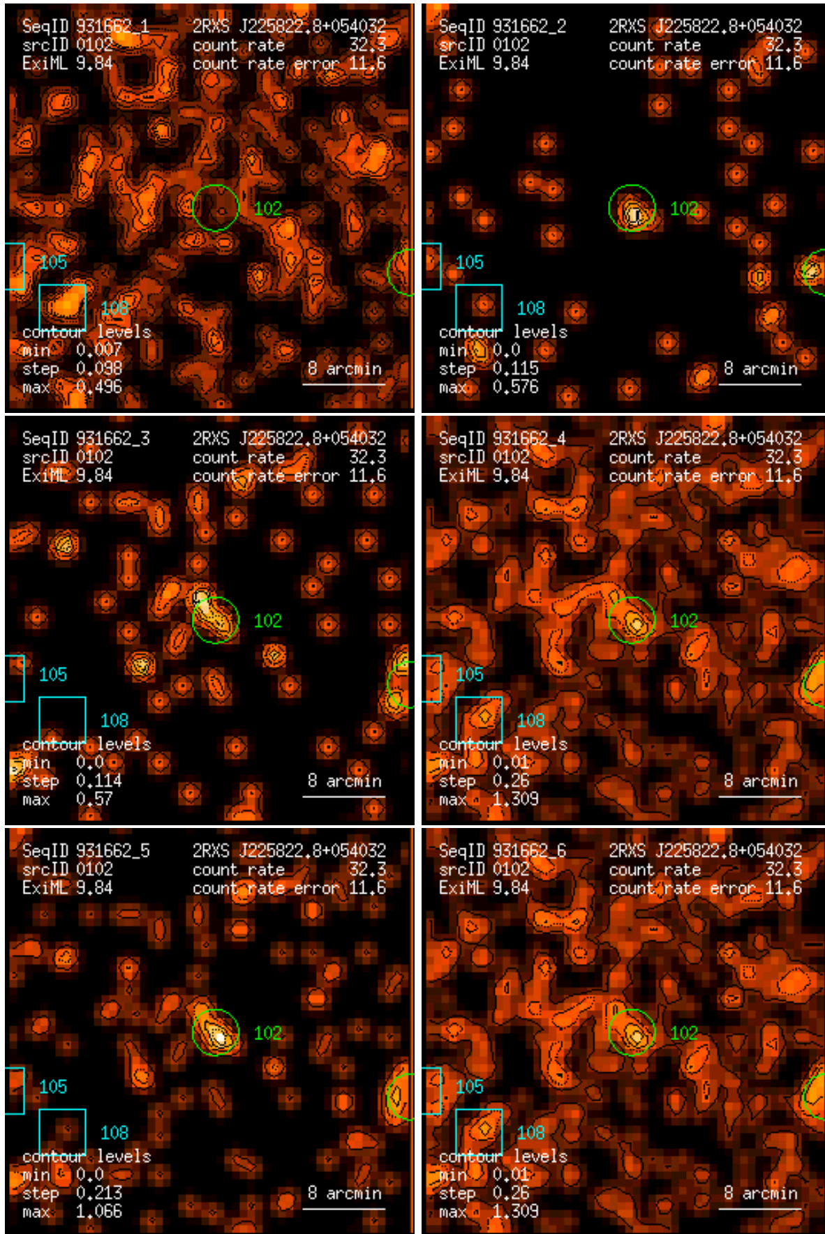
Figure 102: RASS 931662: detection 0102: band rate images, Gaussian filter: (1) PSPC channels 11 – 41, (2) 52 – 90, (3) 91 – 201, (4) 11 – 235, (5) 52 – 201, (6) 11 – 201. Broad band rates in counts/ks. Band rate contour levels in counts/ks/arcmin 2 .
