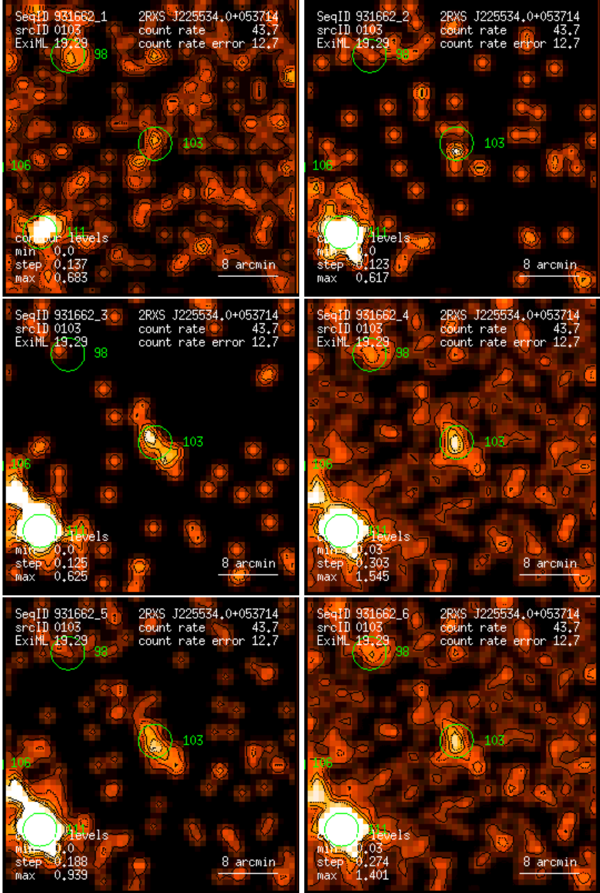
Figure 103: RASS 931662: detection 0103: band rate images, Gaussian filter: (1) PSPC channels 11 – 41, (2) 52 – 90, (3) 91 – 201, (4) 11 – 235, (5) 52 – 201, (6) 11 – 201. Broad band rates in counts/ks. Band rate contour levels in counts/ks/arcmin 2 .
