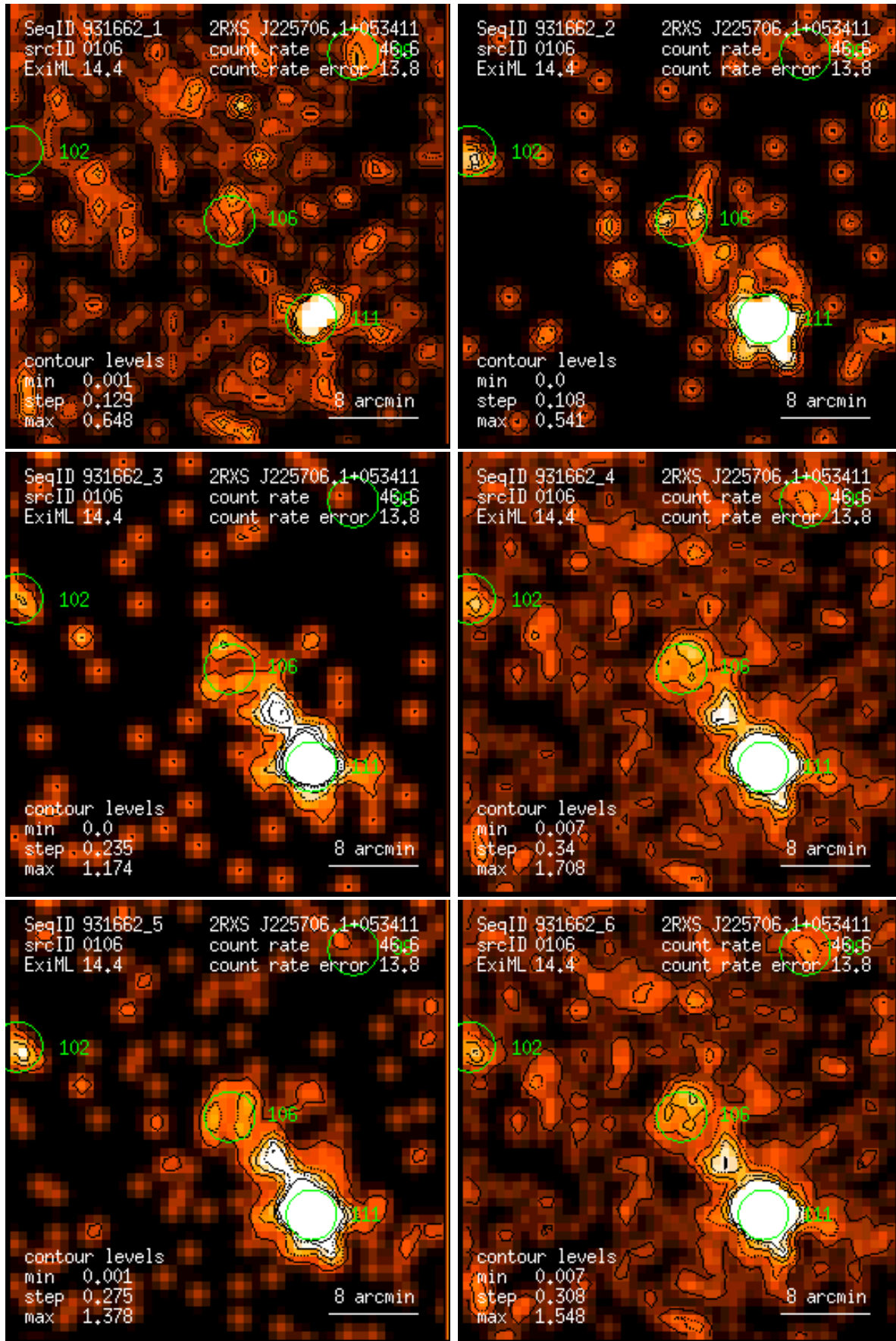
Figure 106: RASS 931662: detection 0106: band rate images, Gaussian filter: (1) PSPC channels 11 – 41, (2) 52 – 90, (3) 91 – 201, (4) 11 – 235, (5) 52 – 201, (6) 11 – 201. Broad band rates in counts/ks. Band rate contour levels in counts/ks/arcmin 2 .
