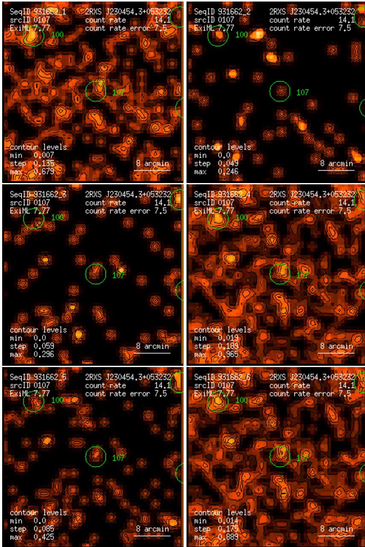
Figure 107: RASS 931662: detection 0107: band rate images, Gaussian filter: (1) PSPC channels 11 – 41, (2) 52 – 90, (3) 91 – 201, (4) 11 – 235, (5) 52 – 201, (6) 11 – 201. Broad band rates in counts/ks. Band rate contour levels in counts/ks/arcmin 2 .
