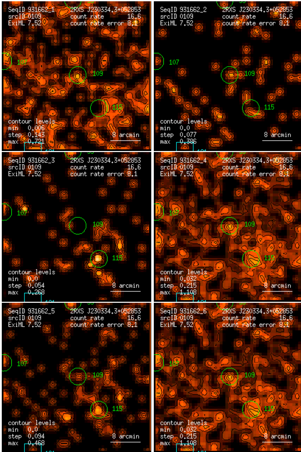
Figure 109: RASS 931662: detection 0109: band rate images, Gaussian filter: (1) PSPC channels 11 – 41, (2) 52 – 90, (3) 91 – 201, (4) 11 – 235, (5) 52 – 201, (6) 11 – 201. Broad band rates in counts/ks. Band rate contour levels in counts/ks/arcmin 2 .
