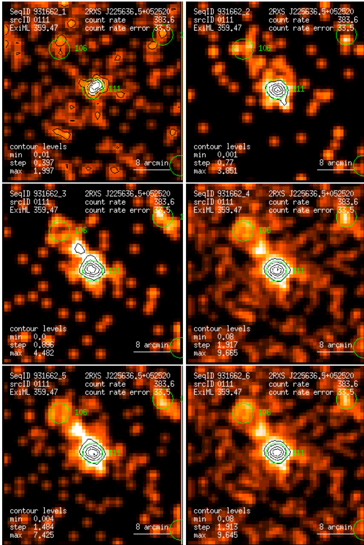
Figure 111: RASS 931662: detection 0111: band rate images, Gaussian filter: (1) PSPC channels 11 – 41, (2) 52 – 90, (3) 91 – 201, (4) 11 – 235, (5) 52 – 201, (6) 11 – 201. Broad band rates in counts/ks. Band rate contour levels in counts/ks/arcmin 2 .
