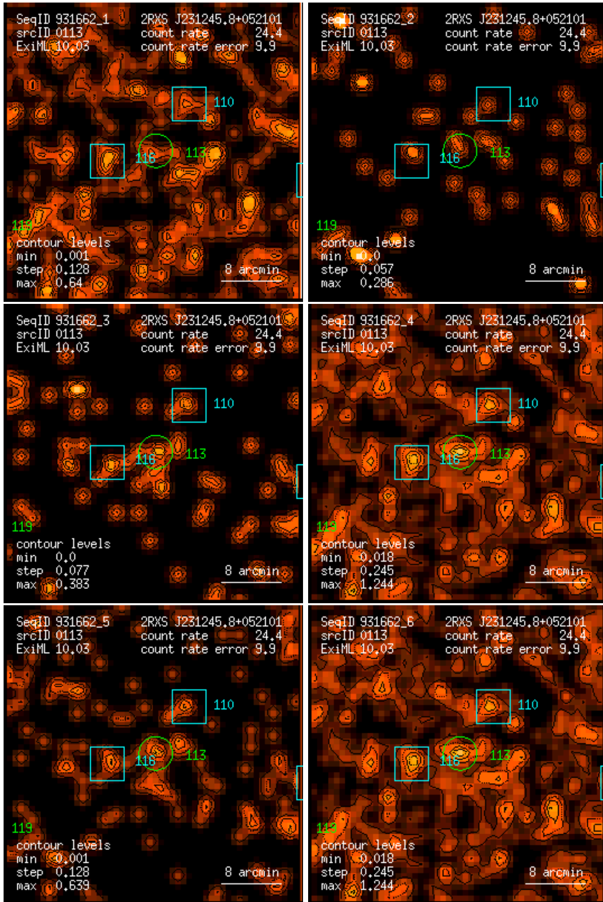
Figure 113: RASS 931662: detection 0113: band rate images, Gaussian filter: (1) PSPC channels 11 – 41, (2) 52 – 90, (3) 91 – 201, (4) 11 – 235, (5) 52 – 201, (6) 11 – 201. Broad band rates in counts/ks. Band rate contour levels in counts/ks/arcmin 2 .
