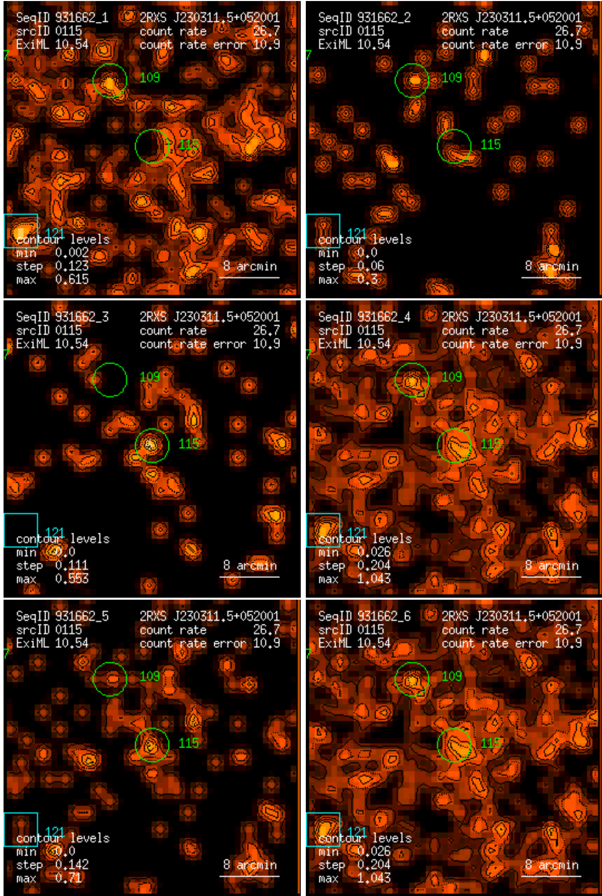
Figure 115: RASS 931662: detection 0115: band rate images, Gaussian filter: (1) PSPC channels 11 – 41, (2) 52 – 90, (3) 91 – 201, (4) 11 – 235, (5) 52 – 201, (6) 11 – 201. Broad band rates in counts/ks. Band rate contour levels in counts/ks/arcmin 2 .
