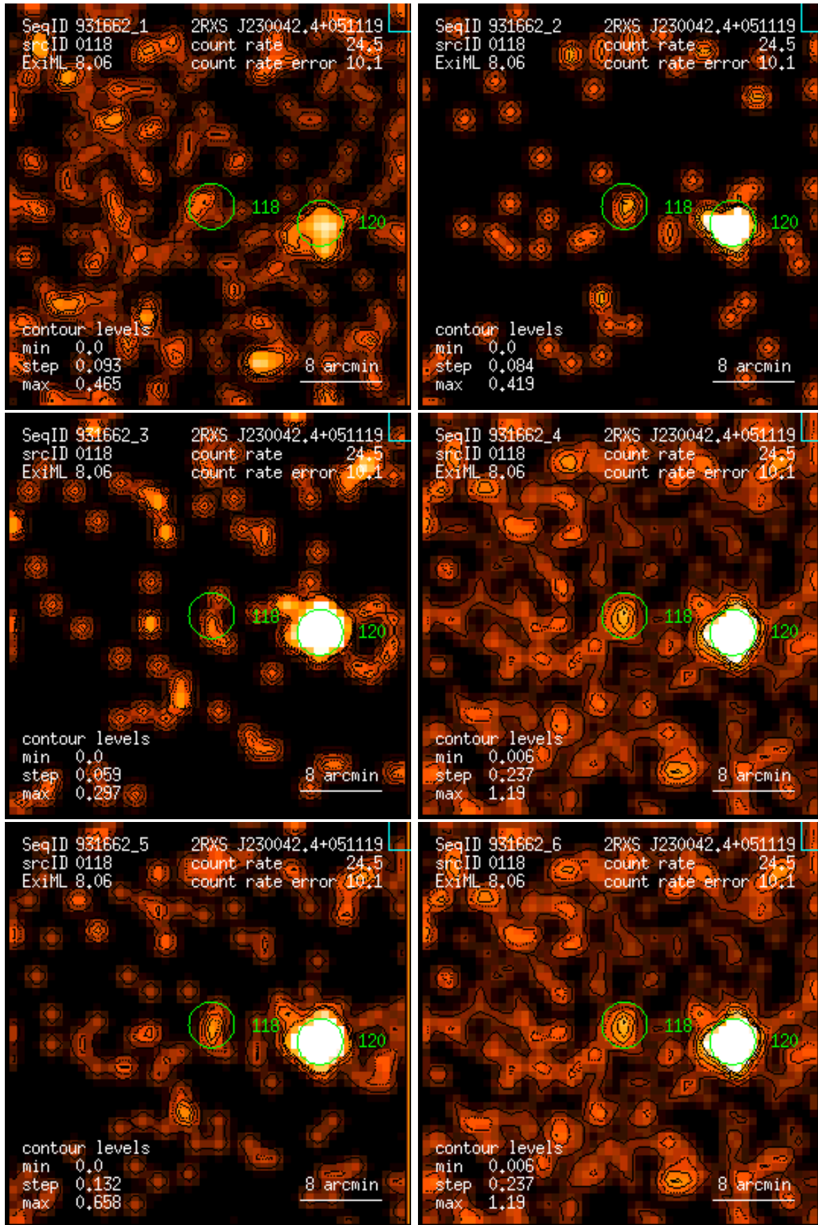
Figure 118: RASS 931662: detection 0118: band rate images, Gaussian filter: (1) PSPC channels 11 – 41, (2) 52 – 90, (3) 91 – 201, (4) 11 – 235, (5) 52 – 201, (6) 11 – 201. Broad band rates in counts/ks. Band rate contour levels in counts/ks/arcmin 2 .
