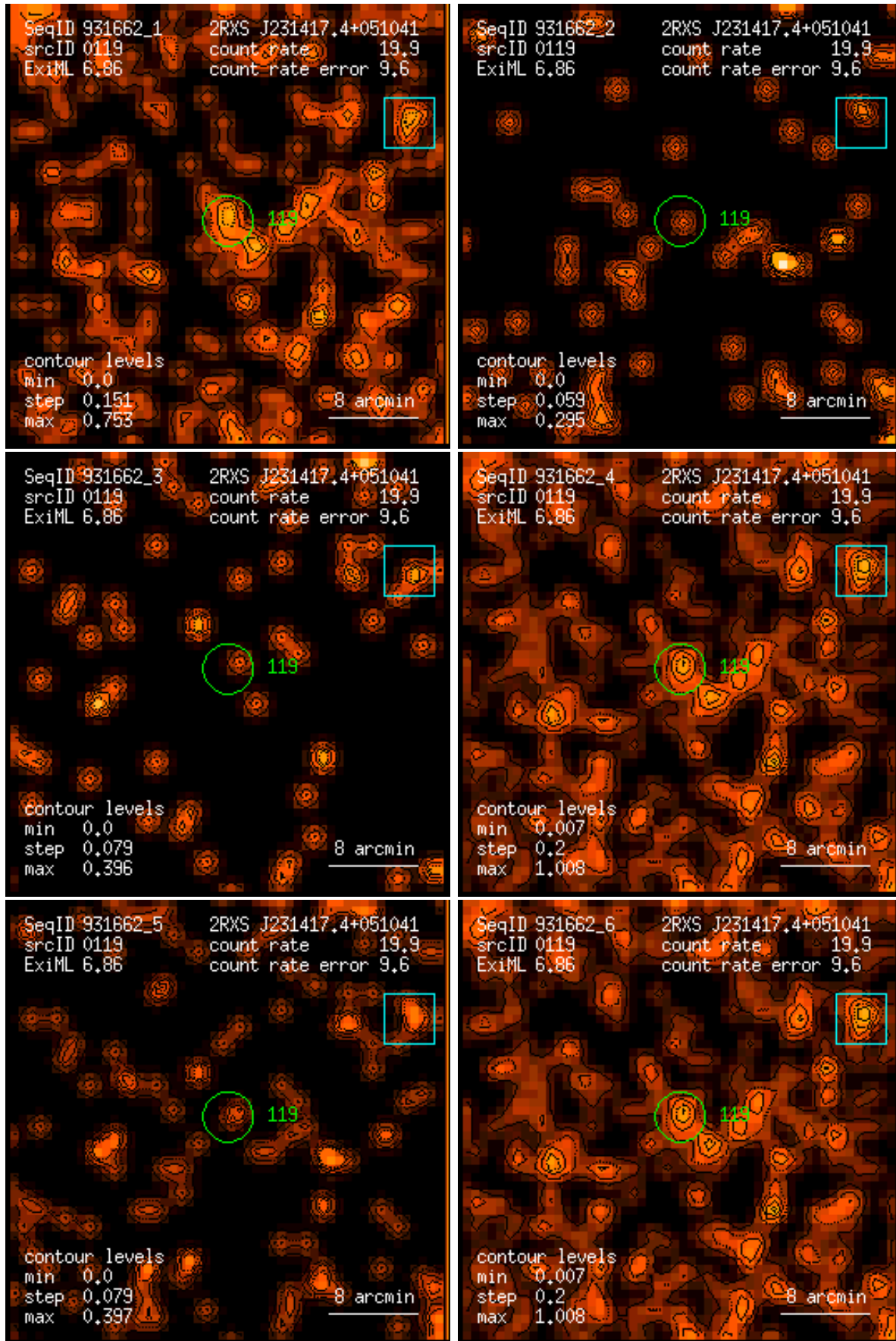
Figure 119: RASS 931662: detection 0119: band rate images, Gaussian filter: (1) PSPC channels 11 – 41, (2) 52 – 90, (3) 91 – 201, (4) 11 – 235, (5) 52 – 201, (6) 11 – 201. Broad band rates in counts/ks. Band rate contour levels in counts/ks/arcmin 2 .
