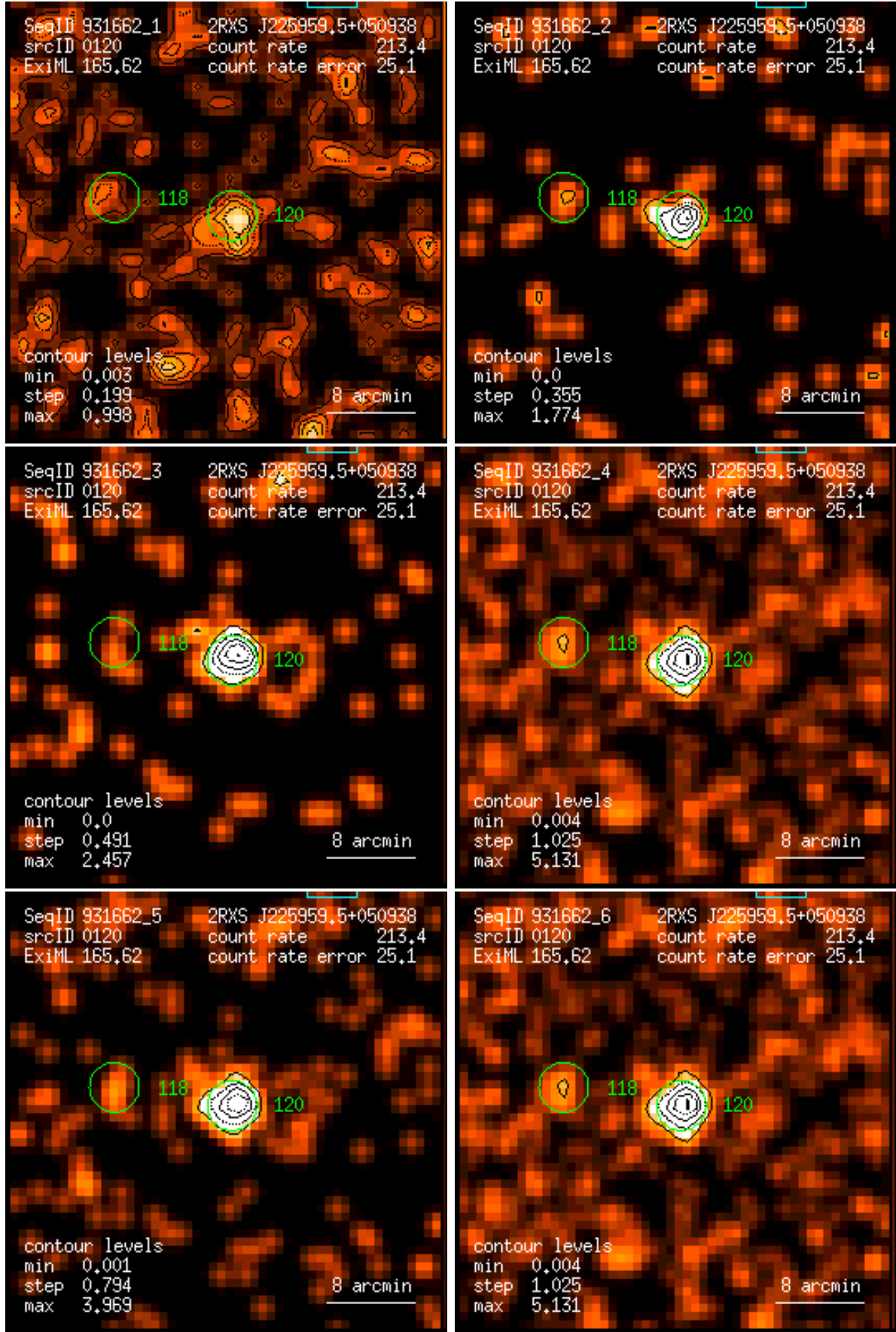
Figure 120: RASS 931662: detection 0120: band rate images, Gaussian filter: (1) PSPC channels 11 – 41, (2) 52 – 90, (3) 91 – 201, (4) 11 – 235, (5) 52 – 201, (6) 11 – 201. Broad band rates in counts/ks. Band rate contour levels in counts/ks/arcmin 2 .
