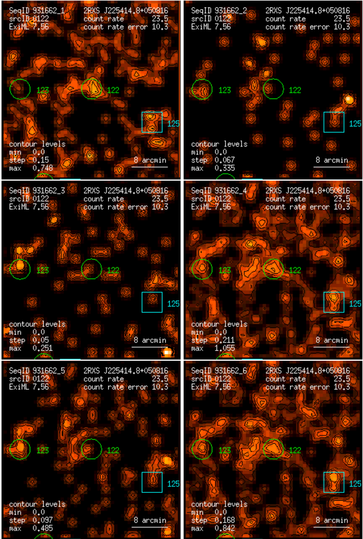
Figure 122: RASS 931662: detection 0122: band rate images, Gaussian filter: (1) PSPC channels 11 – 41, (2) 52 – 90, (3) 91 – 201, (4) 11 – 235, (5) 52 – 201, (6) 11 – 201. Broad band rates in counts/ks. Band rate contour levels in counts/ks/arcmin 2 .
