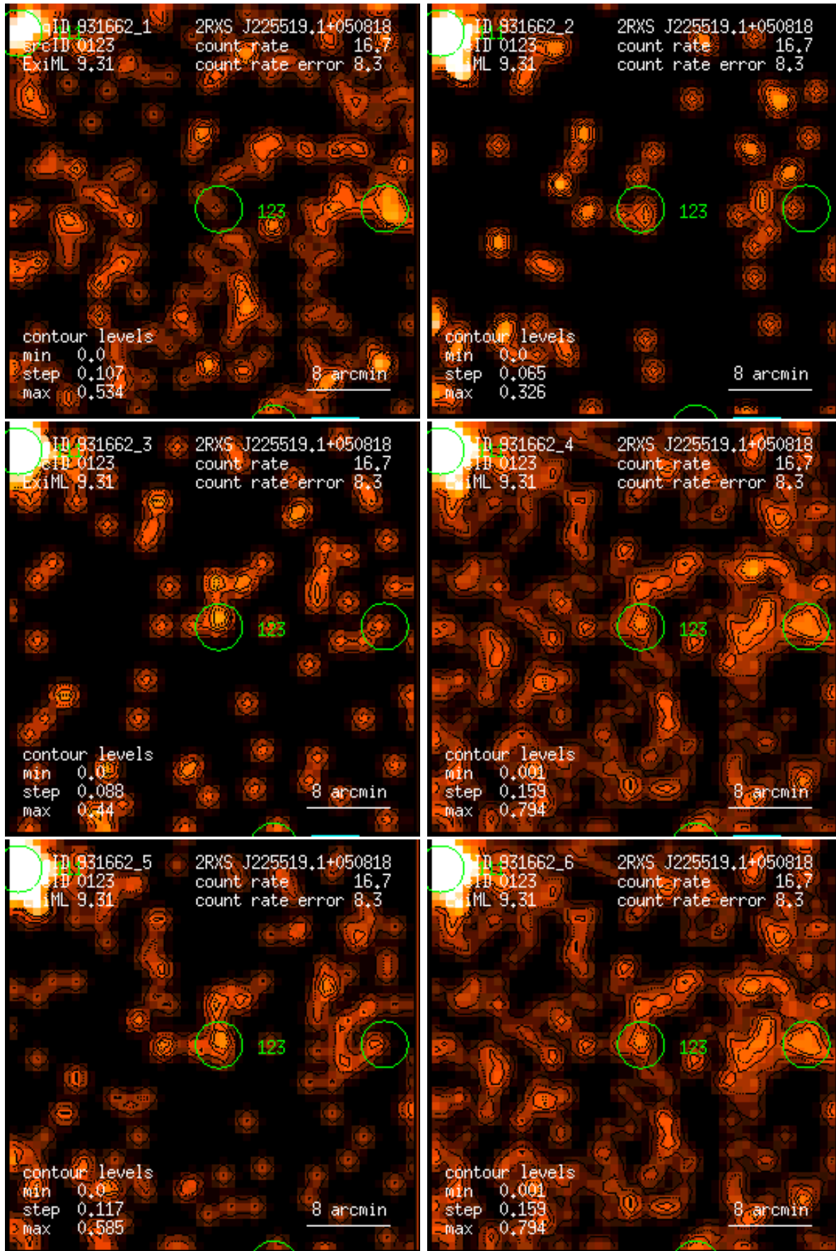
Figure 123: RASS 931662: detection 0123: band rate images, Gaussian filter: (1) PSPC channels 11 – 41, (2) 52 – 90, (3) 91 – 201, (4) 11 – 235, (5) 52 – 201, (6) 11 – 201. Broad band rates in counts/ks. Band rate contour levels in counts/ks/arcmin 2 .
