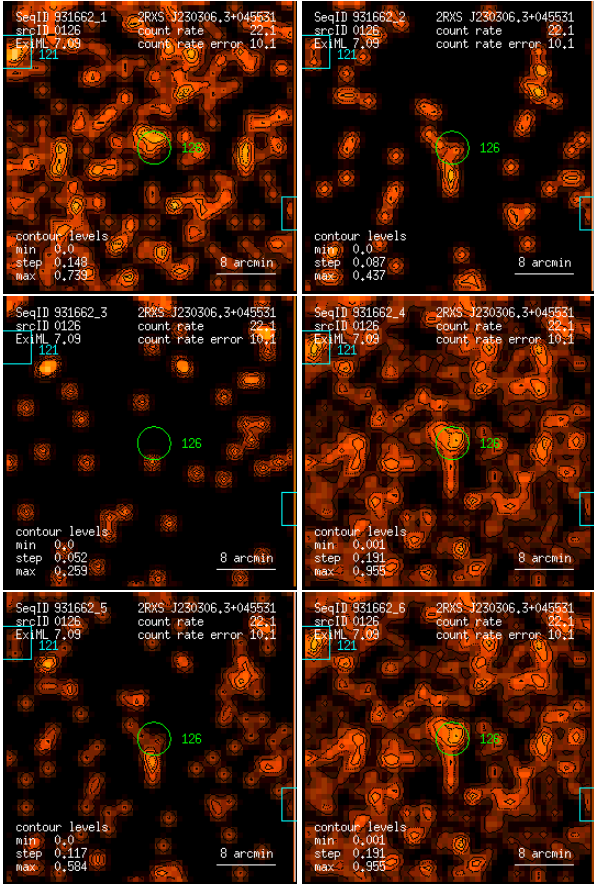
Figure 126: RASS 931662: detection 0126: band rate images, Gaussian filter: (1) PSPC channels 11 – 41, (2) 52 – 90, (3) 91 – 201, (4) 11 – 235, (5) 52 – 201, (6) 11 – 201. Broad band rates in counts/ks. Band rate contour levels in counts/ks/arcmin 2 .
