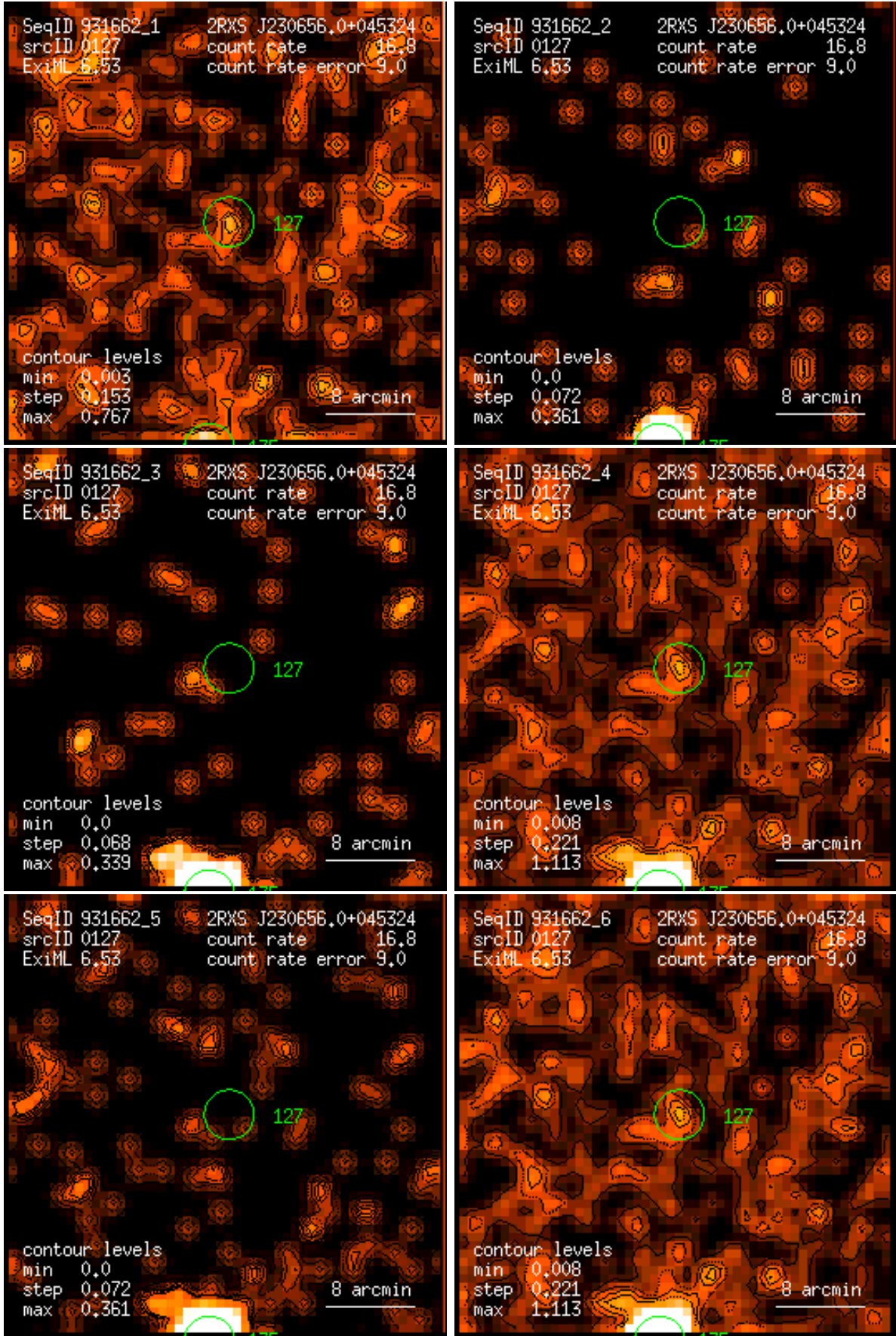
Figure 127: RASS 931662: detection 0127: band rate images, Gaussian filter: (1) PSPC channels 11 – 41, (2) 52 – 90, (3) 91 – 201, (4) 11 – 235, (5) 52 – 201, (6) 11 – 201. Broad band rates in counts/ks. Band rate contour levels in counts/ks/arcmin 2 .
