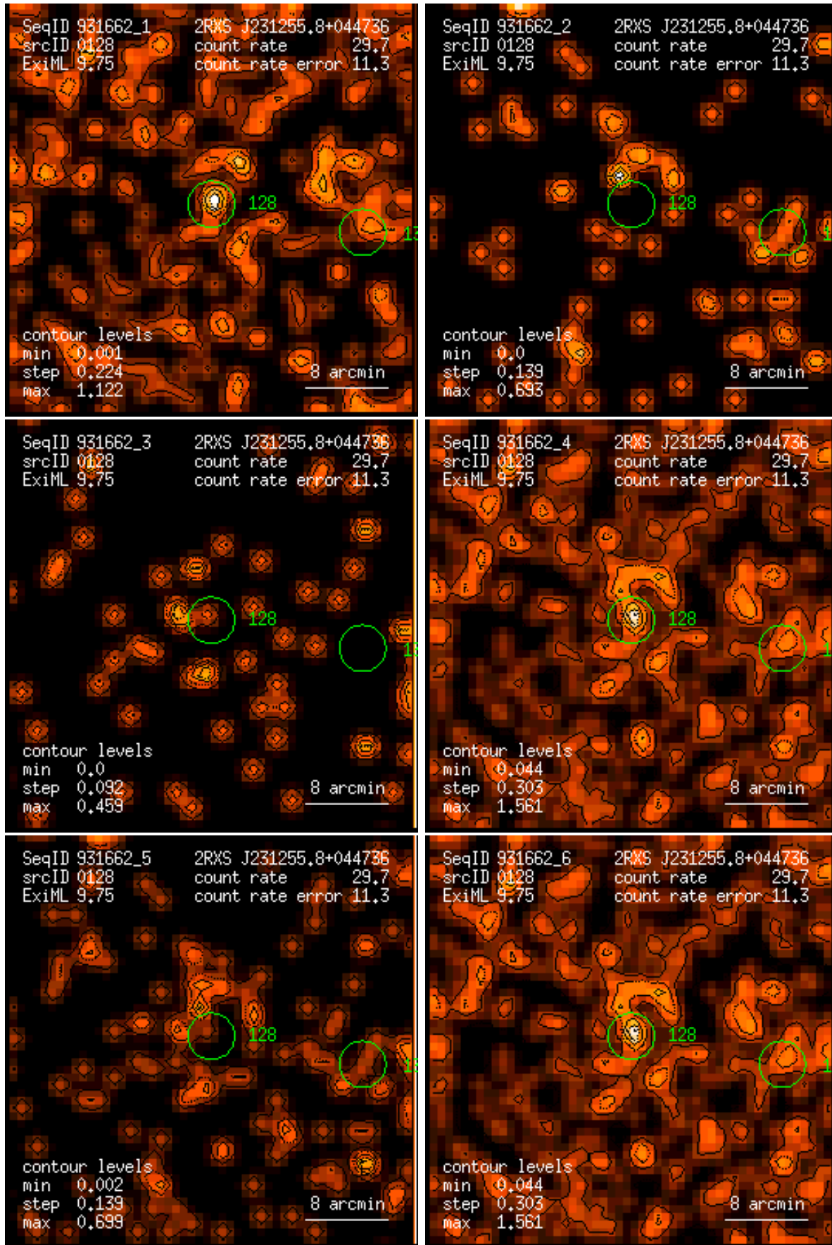
Figure 128: RASS 931662: detection 0128: band rate images, Gaussian filter: (1) PSPC channels 11 – 41, (2) 52 – 90, (3) 91 – 201, (4) 11 – 235, (5) 52 – 201, (6) 11 – 201. Broad band rates in counts/ks. Band rate contour levels in counts/ks/arcmin 2 .
