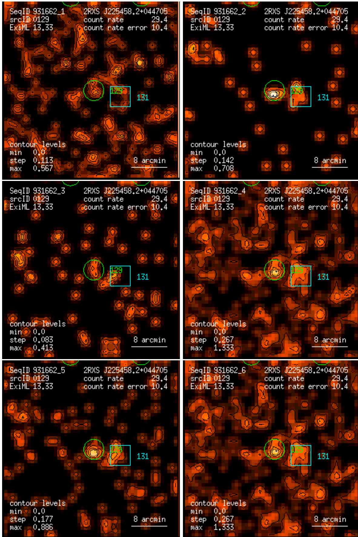
Figure 129: RASS 931662: detection 0129: band rate images, Gaussian filter: (1) PSPC channels 11 – 41, (2) 52 – 90, (3) 91 – 201, (4) 11 – 235, (5) 52 – 201, (6) 11 – 201. Broad band rates in counts/ks. Band rate contour levels in counts/ks/arcmin 2 .
