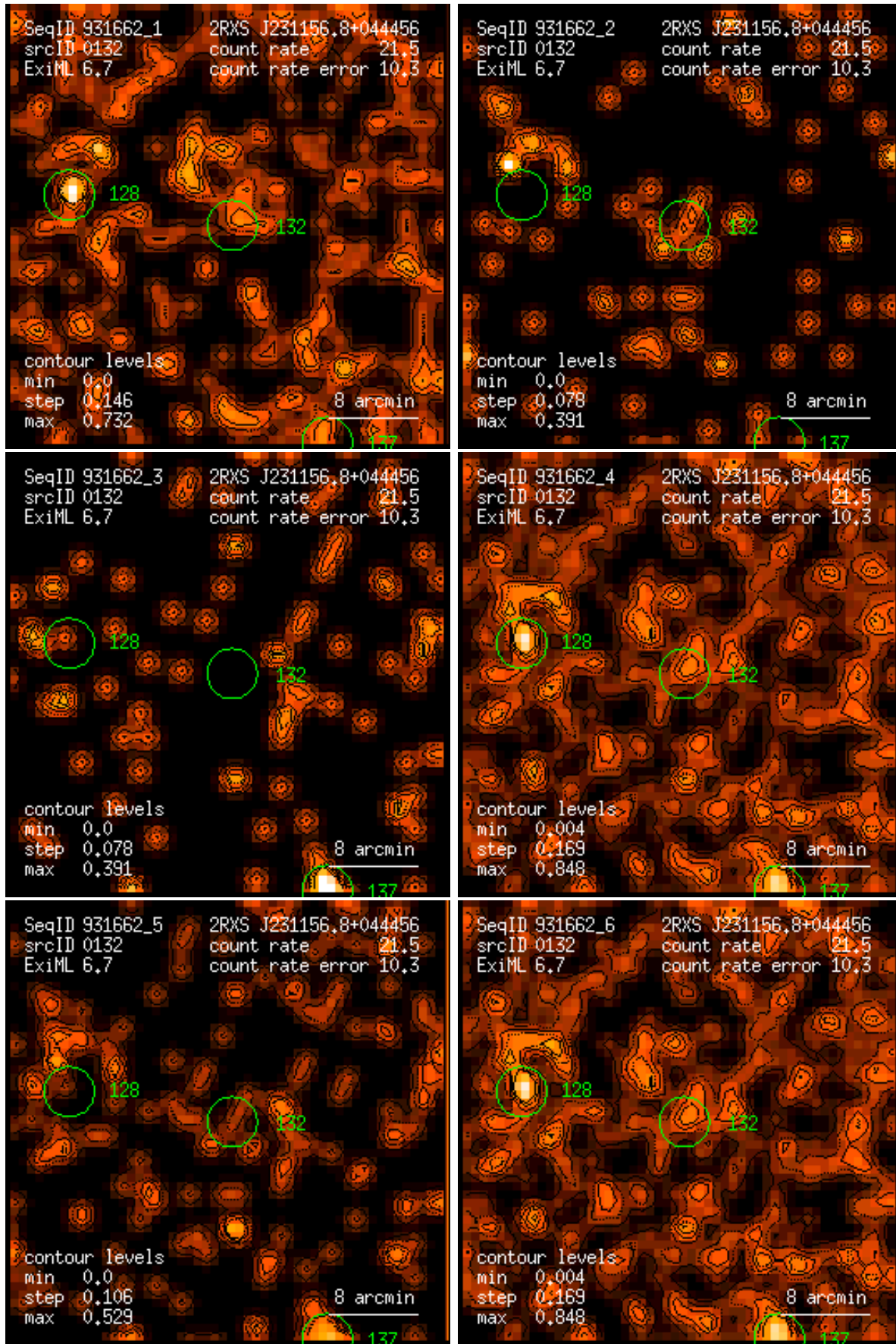
Figure 132: RASS 931662: detection 0132: band rate images, Gaussian filter: (1) PSPC channels 11 – 41, (2) 52 – 90, (3) 91 – 201, (4) 11 – 235, (5) 52 – 201, (6) 11 – 201. Broad band rates in counts/ks. Band rate contour levels in counts/ks/arcmin 2 .
